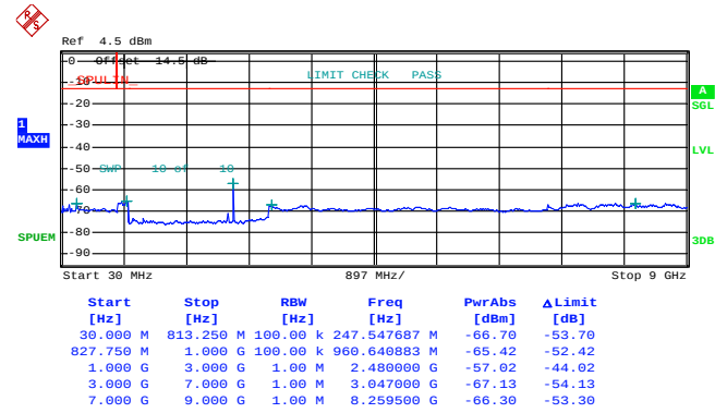
Conducted Emission Plot between on Channel 476 (817.9MHz)
