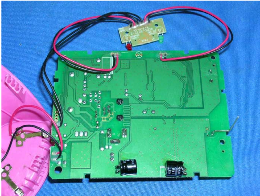
Base Unit Main PCB and LED solder side
