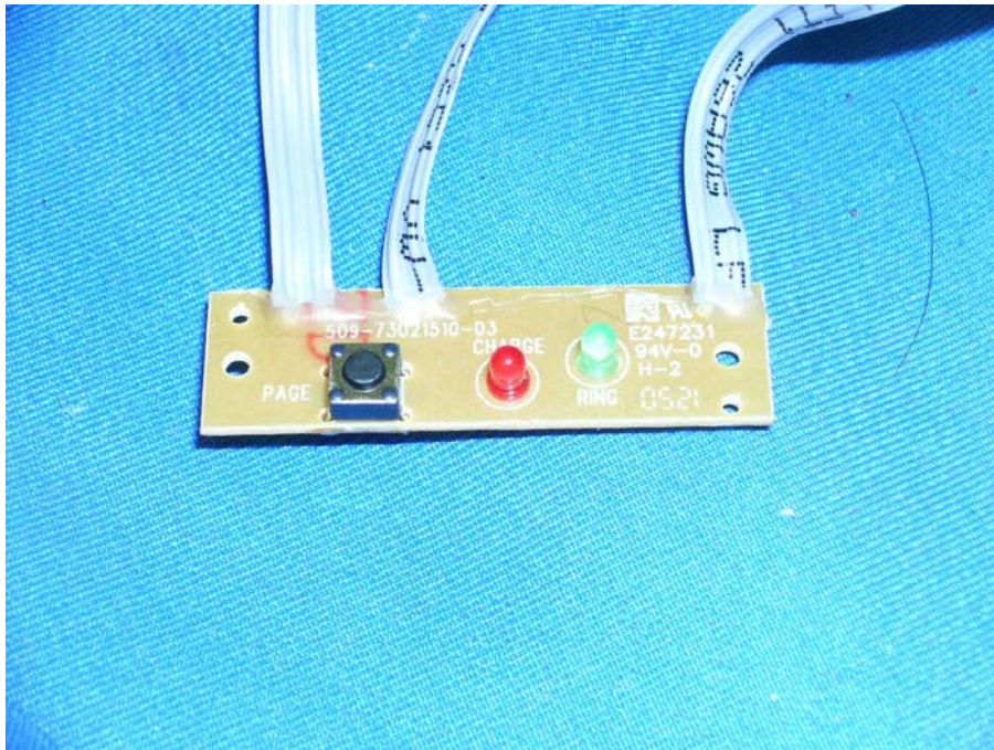
Base Page Key and LED front side
