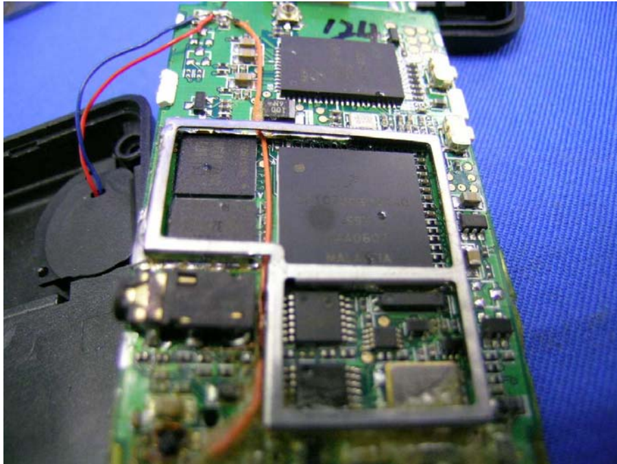
WiFi Phone Oscillator PCB comp side (View 2)
