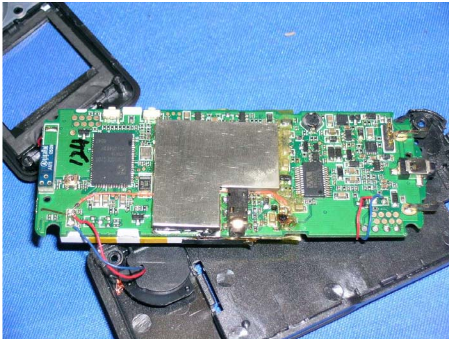
WiFi Phone Main PCB comp side
