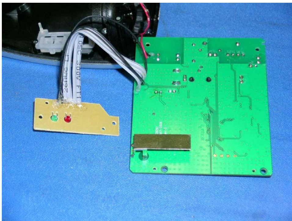
Base Unit Main PCB, Keypad & LED solder side
