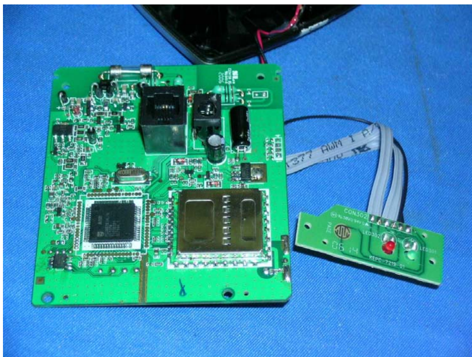
Base Unit Main PCB, Keypad & LED comp side
