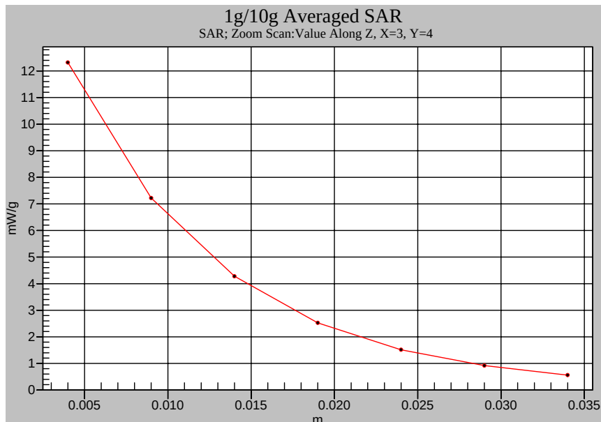
Body-Tissue-Simulating-Liquid 2GHz
