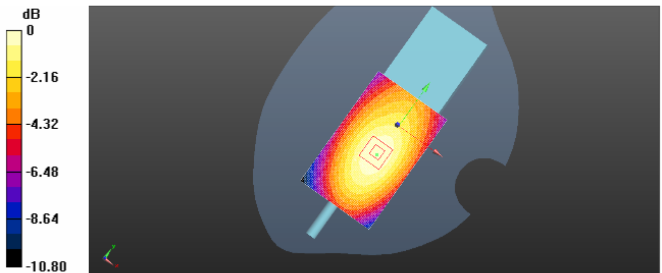
Plot 4: Body-worn for FRS Analog With Belt Clip and Headset Front towards Ground 467.6375 MHz
