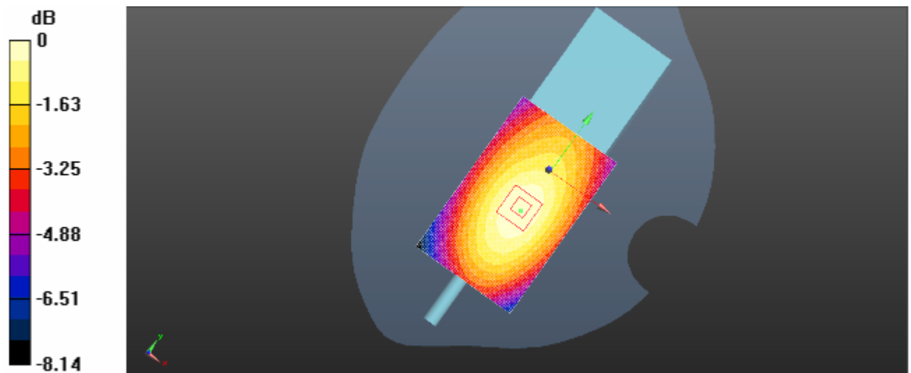
Plot 3: Body-worn for GMRS Analog With Belt Clip and Headset Front towards Ground 462.6375 MHz
