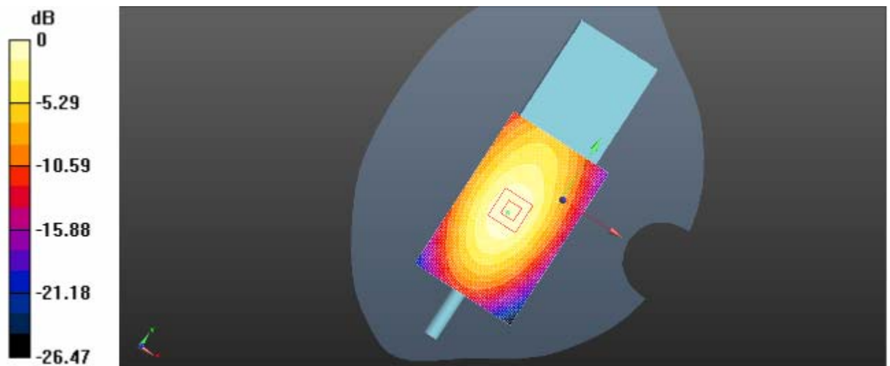
Figure 2: Face held for FRS Analog Front towards Phantom 467.6375 MHz
