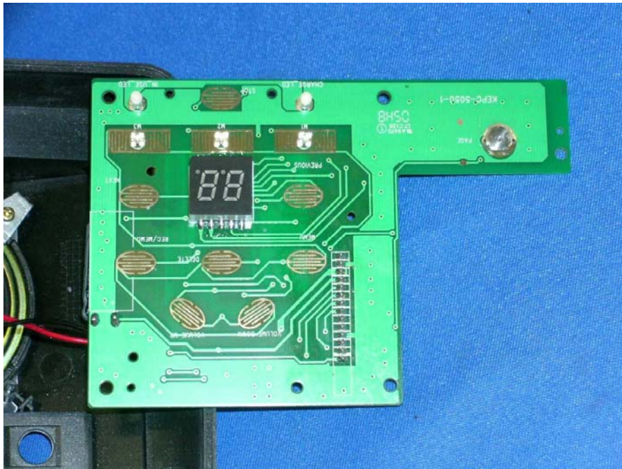
Base DAM keypad front side
