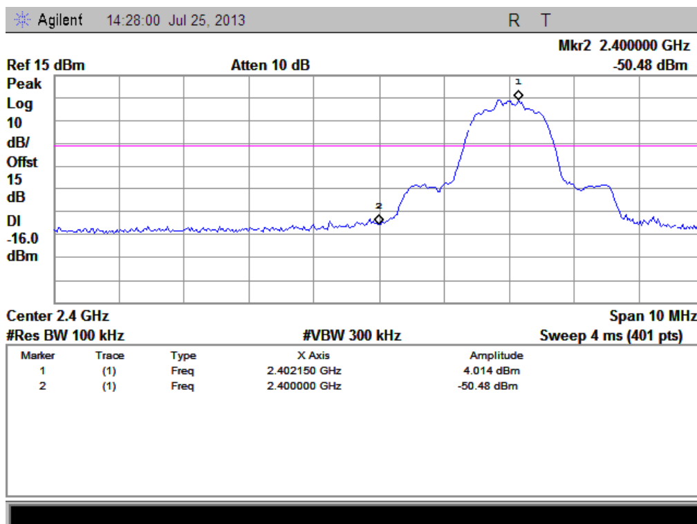
(Channel = 0, Band Edge with hopping off @ \pi/4 -DQPSK)
