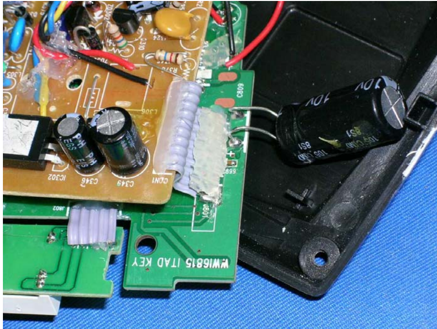
Base Keypad and Display rear side (View 2)
