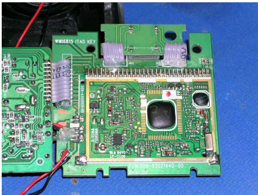
Base Keypad and Display rear side (View 1)
