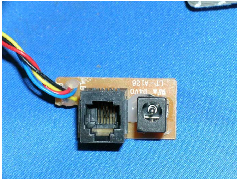
Base AC Jack and Telephone Line Jack front side
