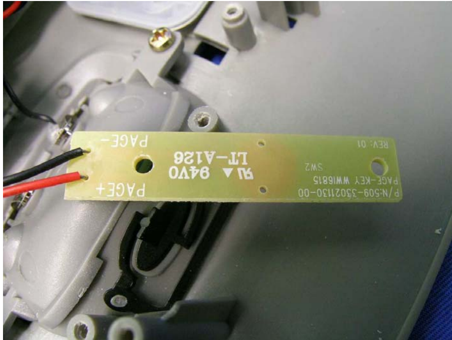
Base Page Key PCB rear side
