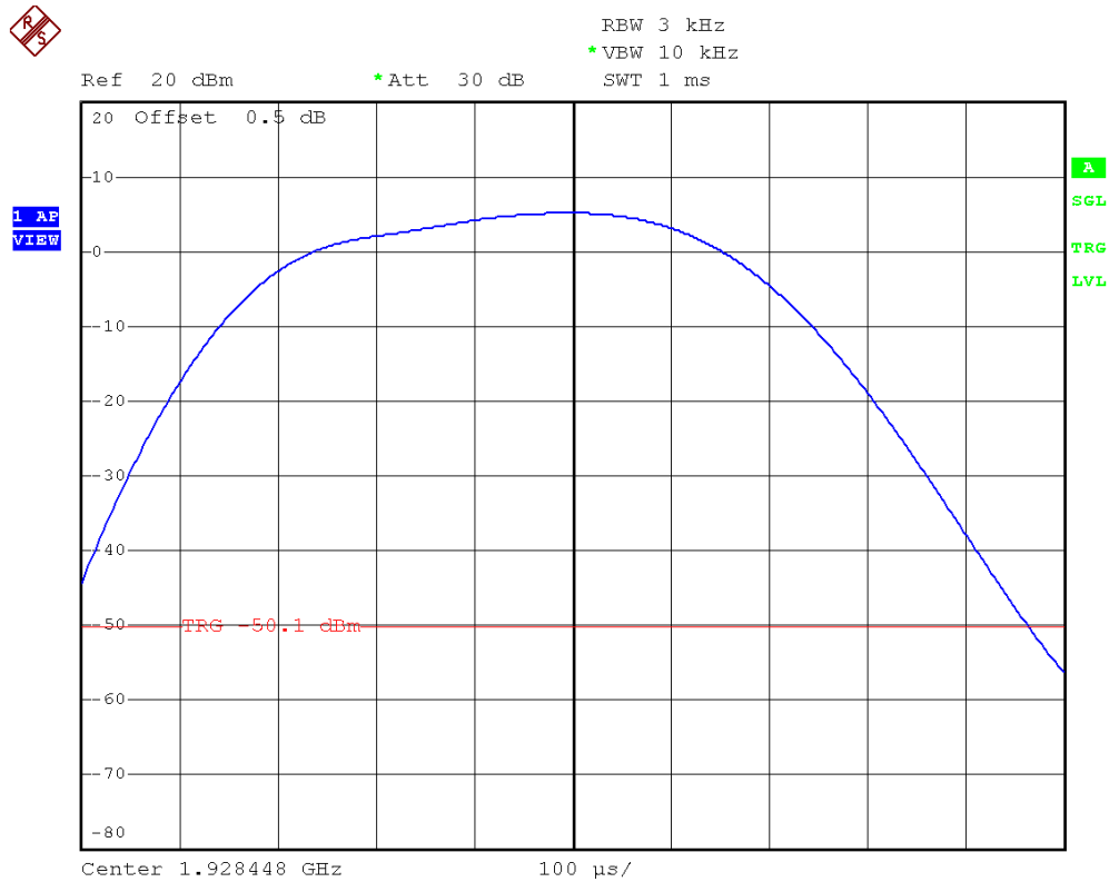
Plot 3B. Highest Channel Power Spectral Density (Traffic Carrier)
