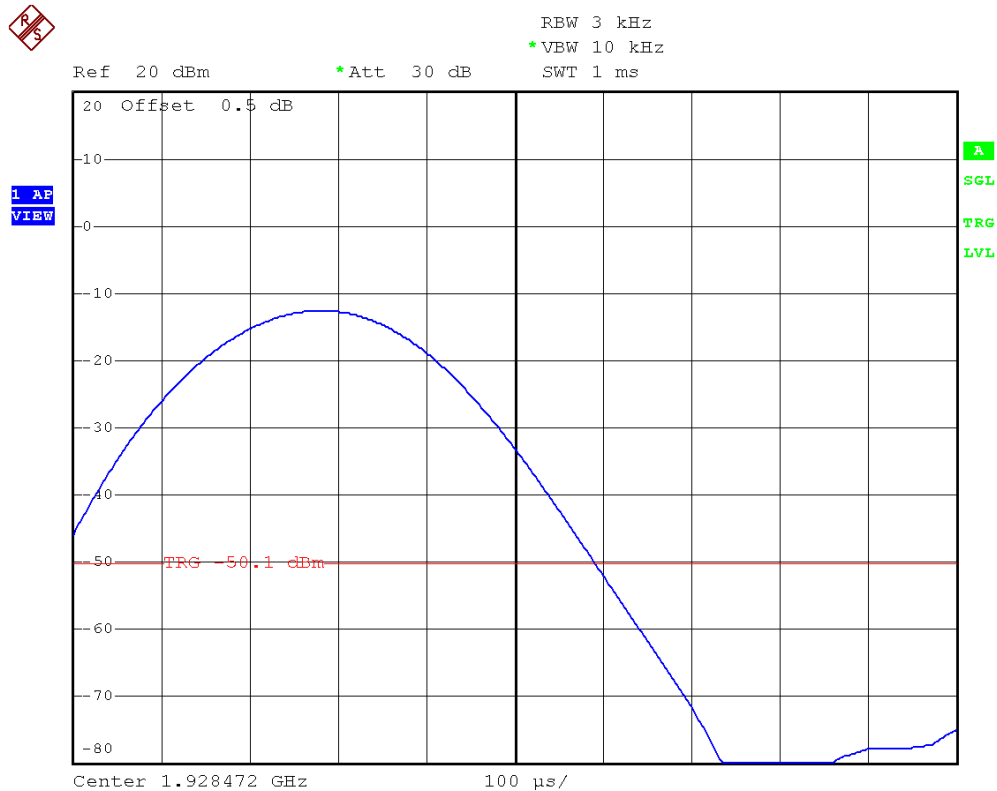
Plot 3D. Highest Channel Power Spectral Density (Dummy Carrier)
