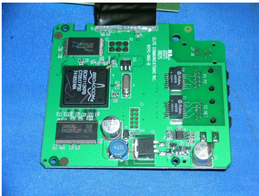
Base Unit another Main PCB comp side
