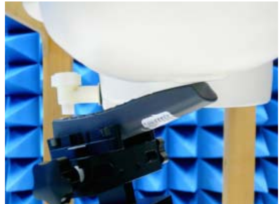
Figure 18.Left Head SAR Test Setup (Tilted)
