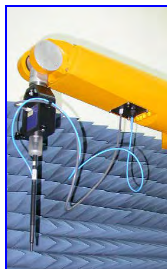
Figure 9. Probe setup on robot
