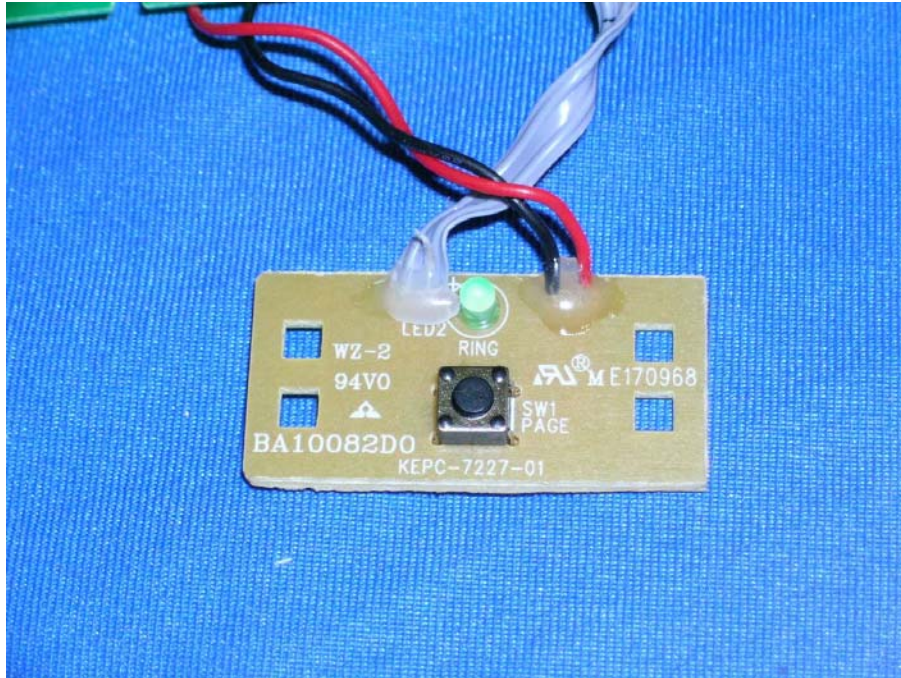
Base LED and Page Key front side
