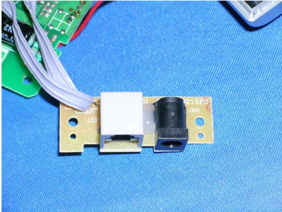
Base Telephone Jack and AC Jack front side
