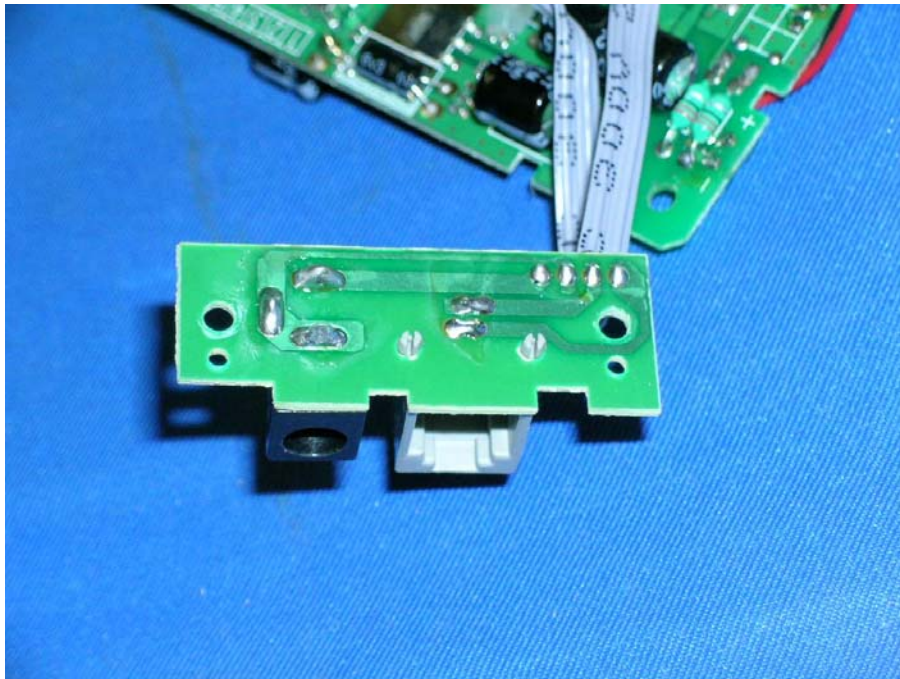
Base Telephone Jack and AC Jack rear side
