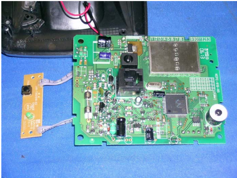
Base Unit Main PCB, Page Key and LED comp side
