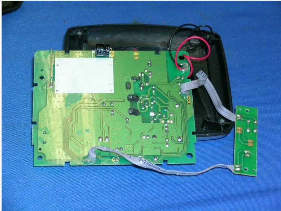
Base Unit Main PCB, Page Key and LED solder side
