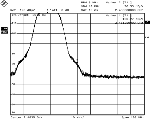
Upper Bandedge - 12dBi Omnidirectional - CH11 - 6Mbps Date: 9.MAY.2006 17:00:14
