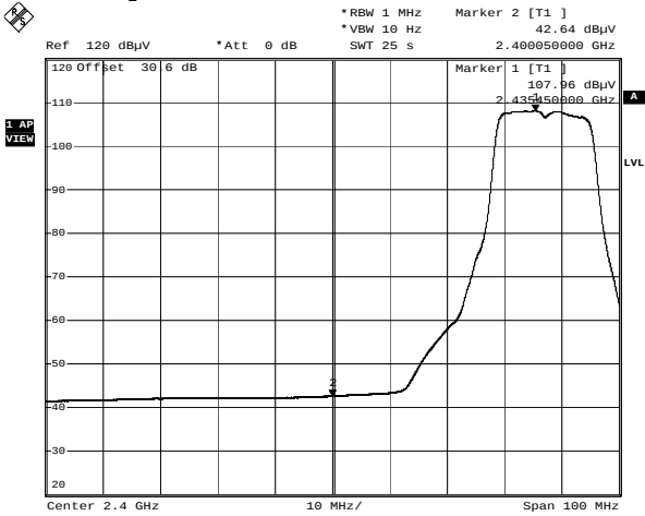
Lower Bandedge - 12dBi Omnidirectional - CH6 - 6Mbps Date: 9.MAY.2006 17:13:25
