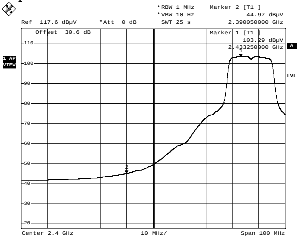
Lower Bandedge - 8dBi Directional - CH6 - 6Mbps Date: 9.MAY.2006 16:01:39
