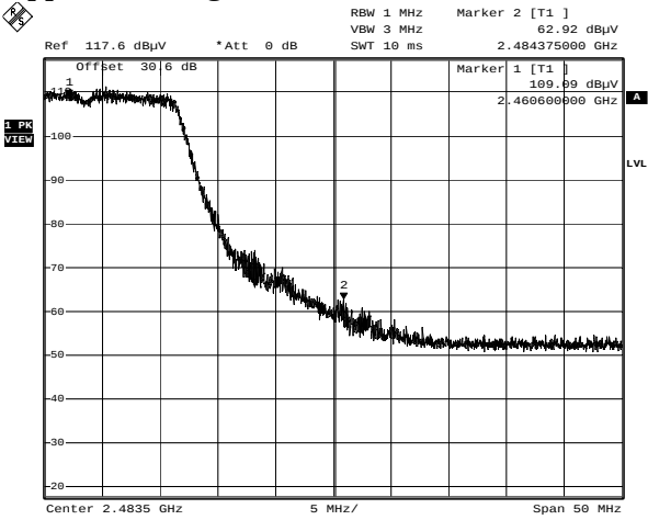
Upper Bandedge - 8dBi Directional - CH11 - 6Mbps Date: 9.MAY.2006 15:57:01
