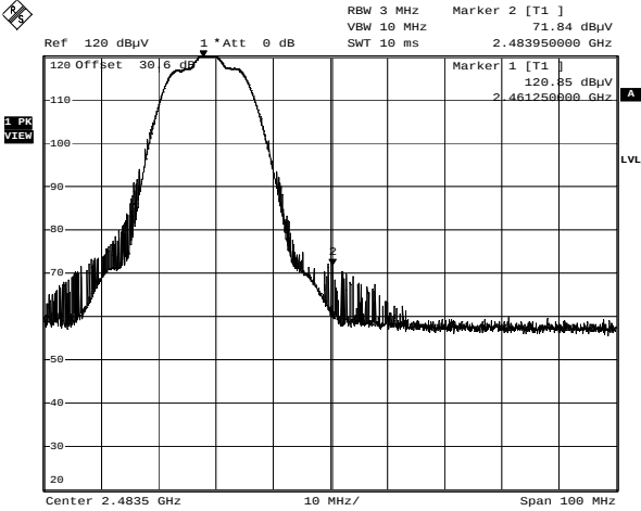
Upper Bandedge - 12dBi Omnidirectional - CH11 - 1Mbps Date: 9.MAY.2006 17:03:05
