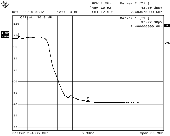
Upper Bandedge - 8dBi Directional - CH11 - 6Mbps Date: 9.MAY.2006 15:58:31
