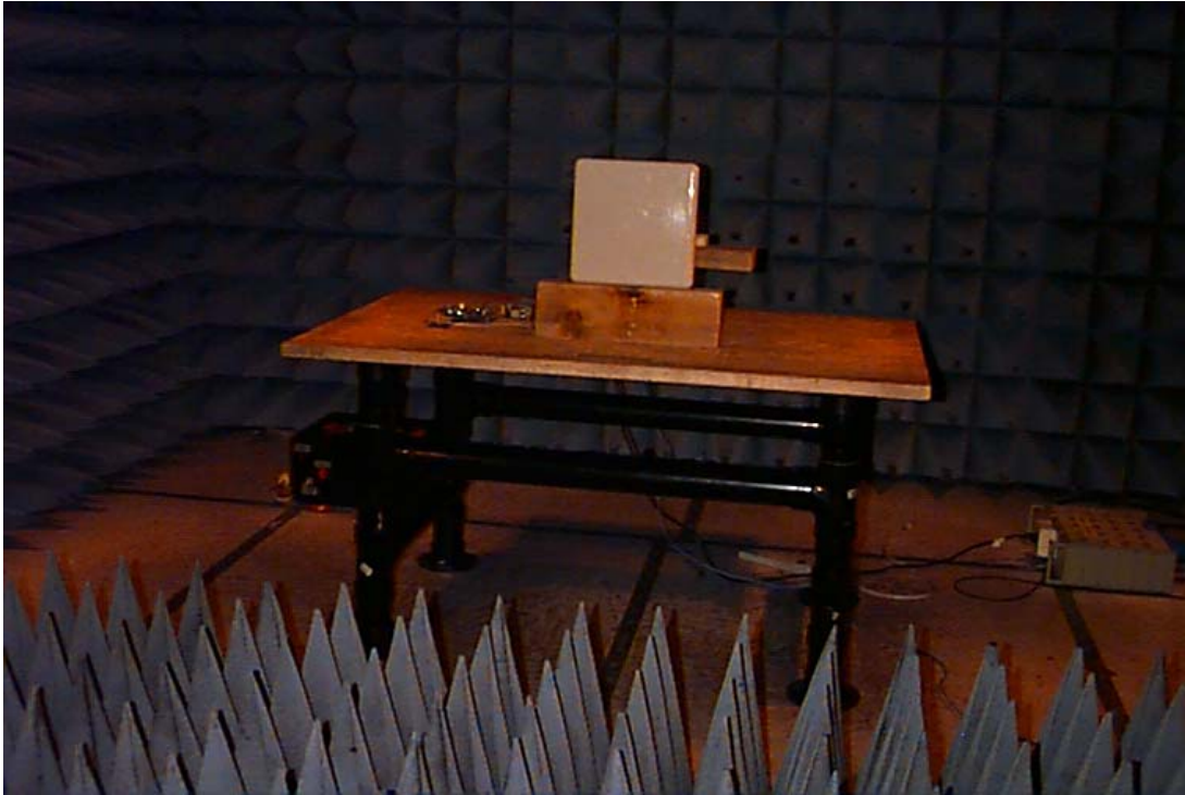
23dBi Huber&Suhner
