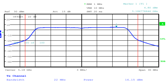
Figure 8.4-2: Sample plot for PSD on 802.11n HT20
