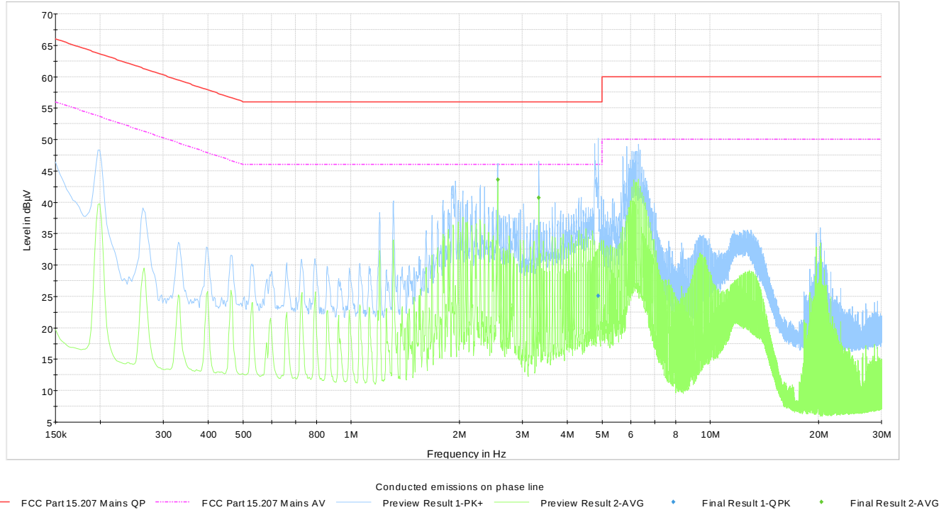
Plot 8.1-1: Conducted emissions on phase line
