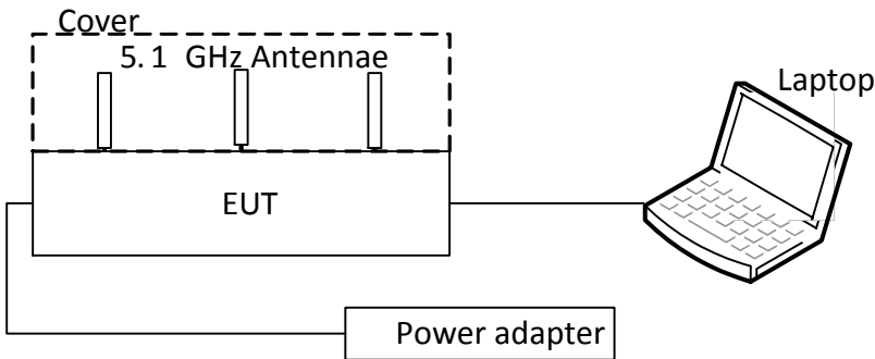
Figure 3.6-1: Setup diagram
