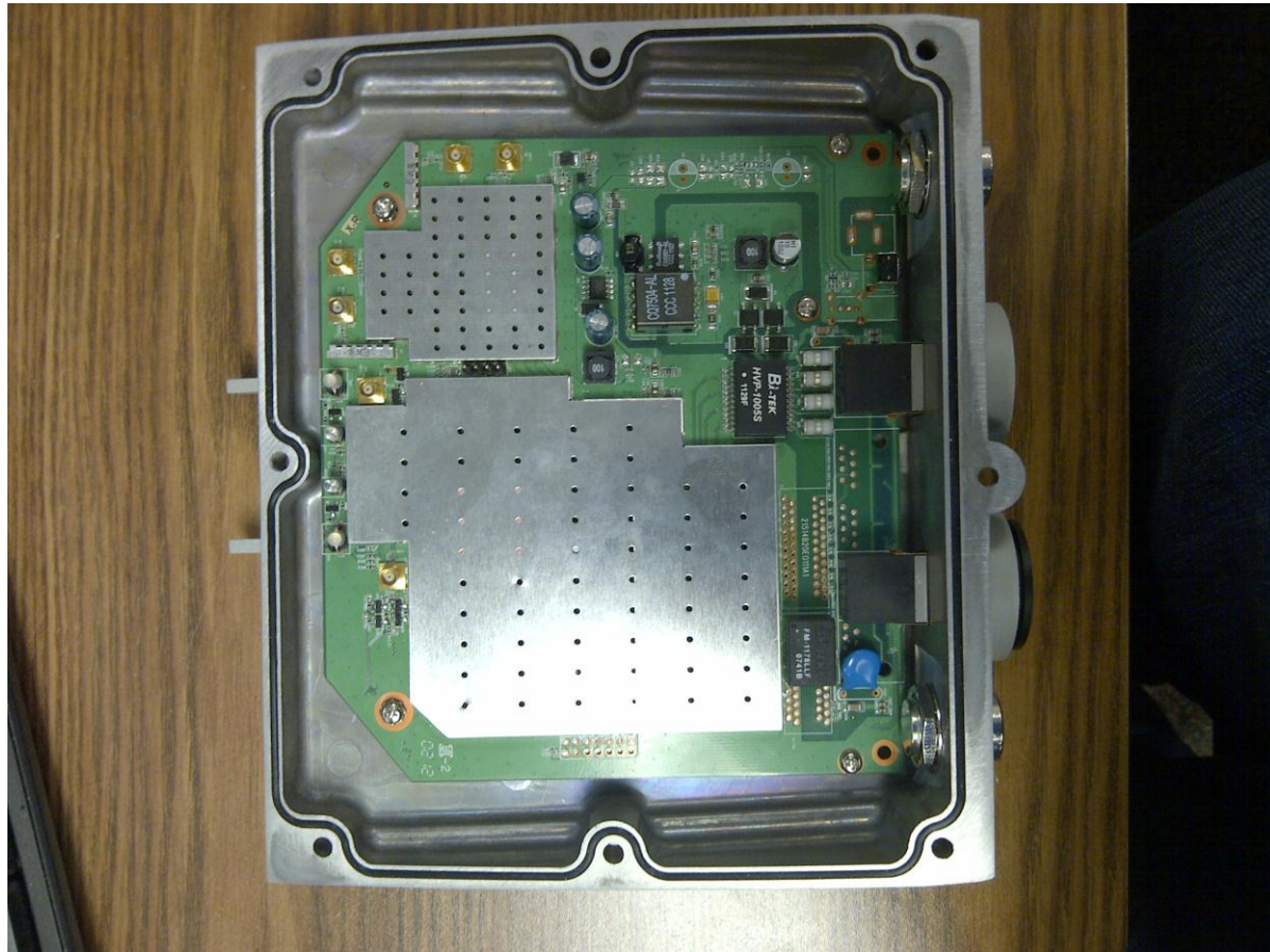
Photo #5 – Main board – component side – with shield
