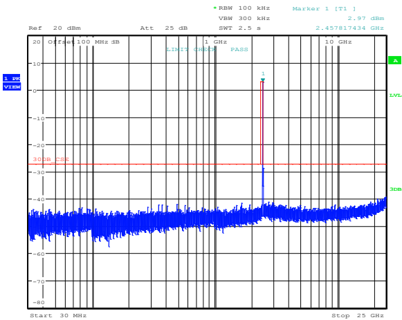
Figure 8.5-9: Conducted spurious emissions for 802.11b, cho, high channel
