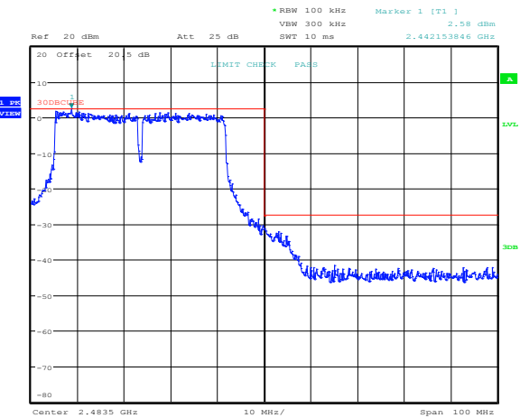
Figure 8.5-34: Conducted upper band edge for 802.11g, cho
