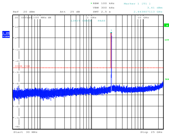
Figure 8.5-10: Conducted spurious emissions for 802.11g, cho, high channel
