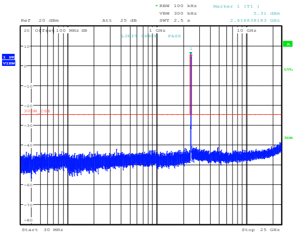
Figure 8.5-1: Conducted spurious emissions for 802.11b, cho, low channel
