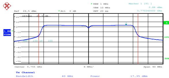
Figure 8.4-3: Output power on 802.11n HT40, sample plot
