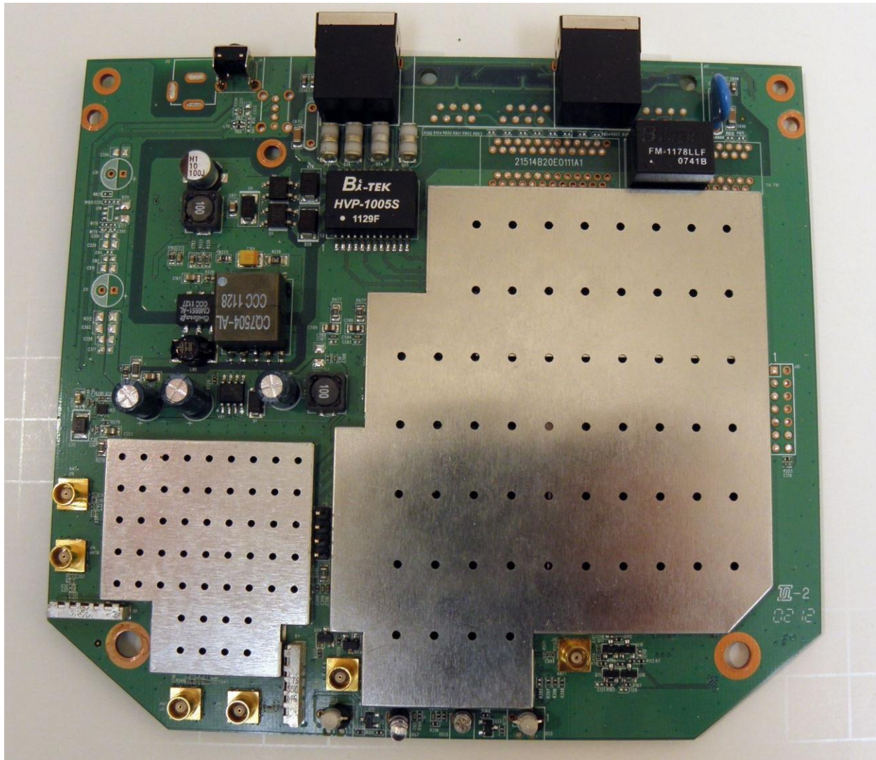
Main board – top with RF shields
