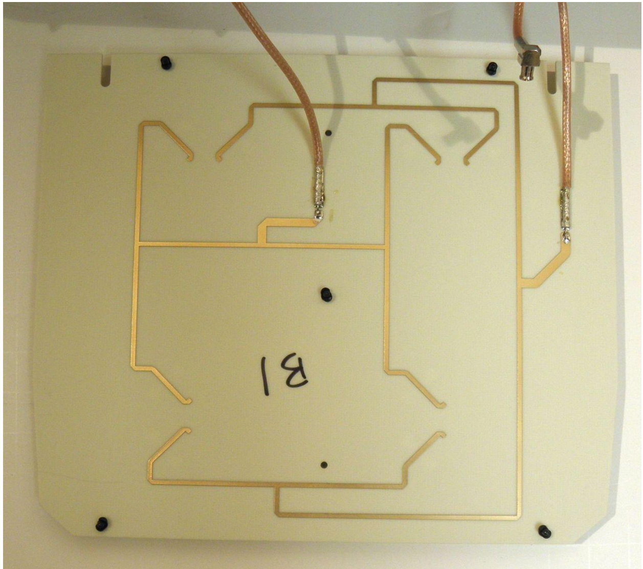
2.4GHz antenna bottom view
