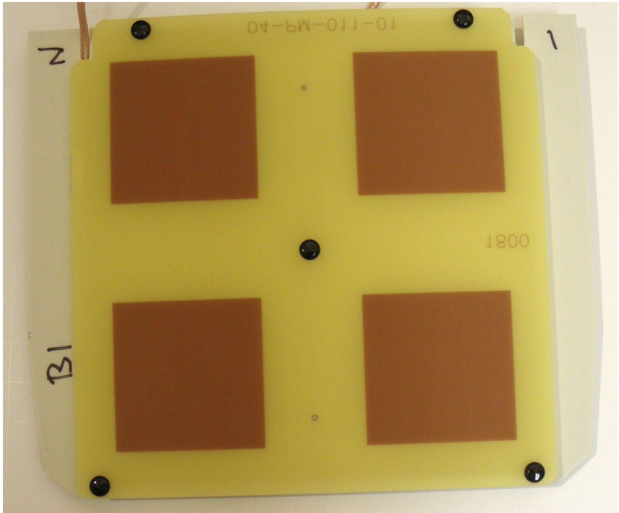
2.4GHz antenna top view
