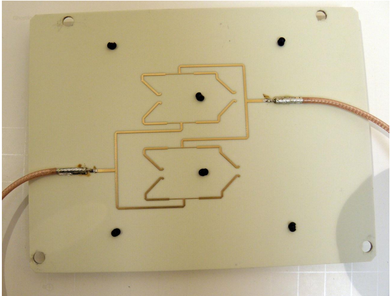
5GHz antenna bottom view
