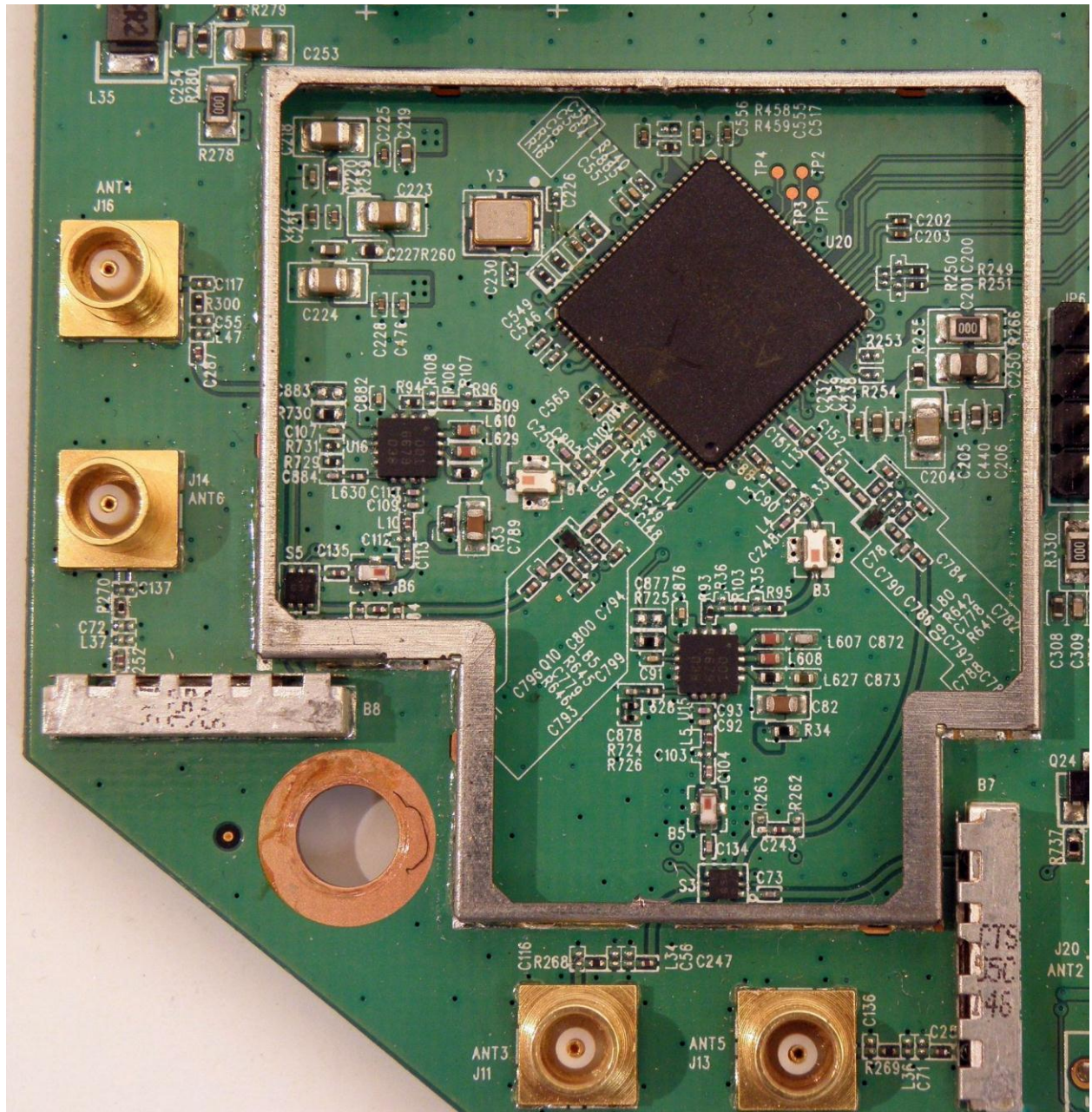
Main board top – RF shield 1 removed
