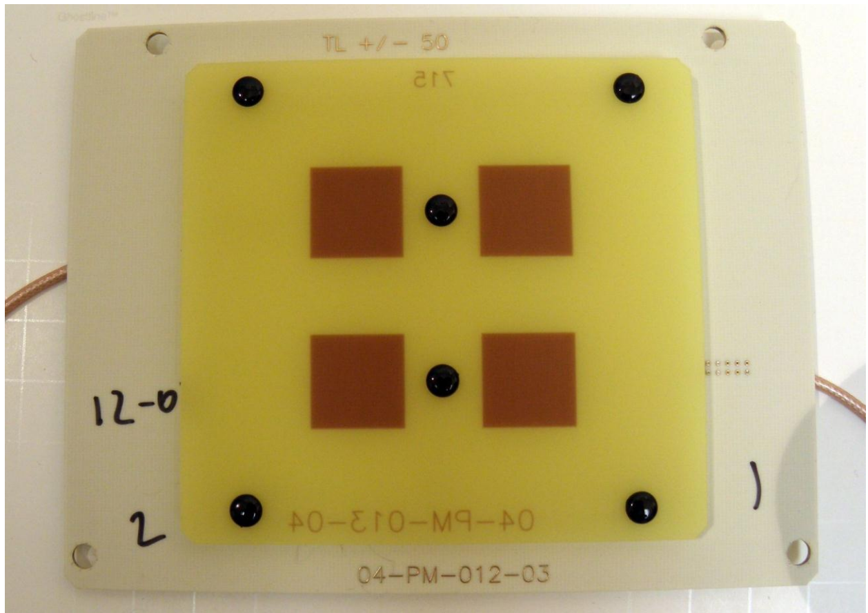
5GHz antenna top view
