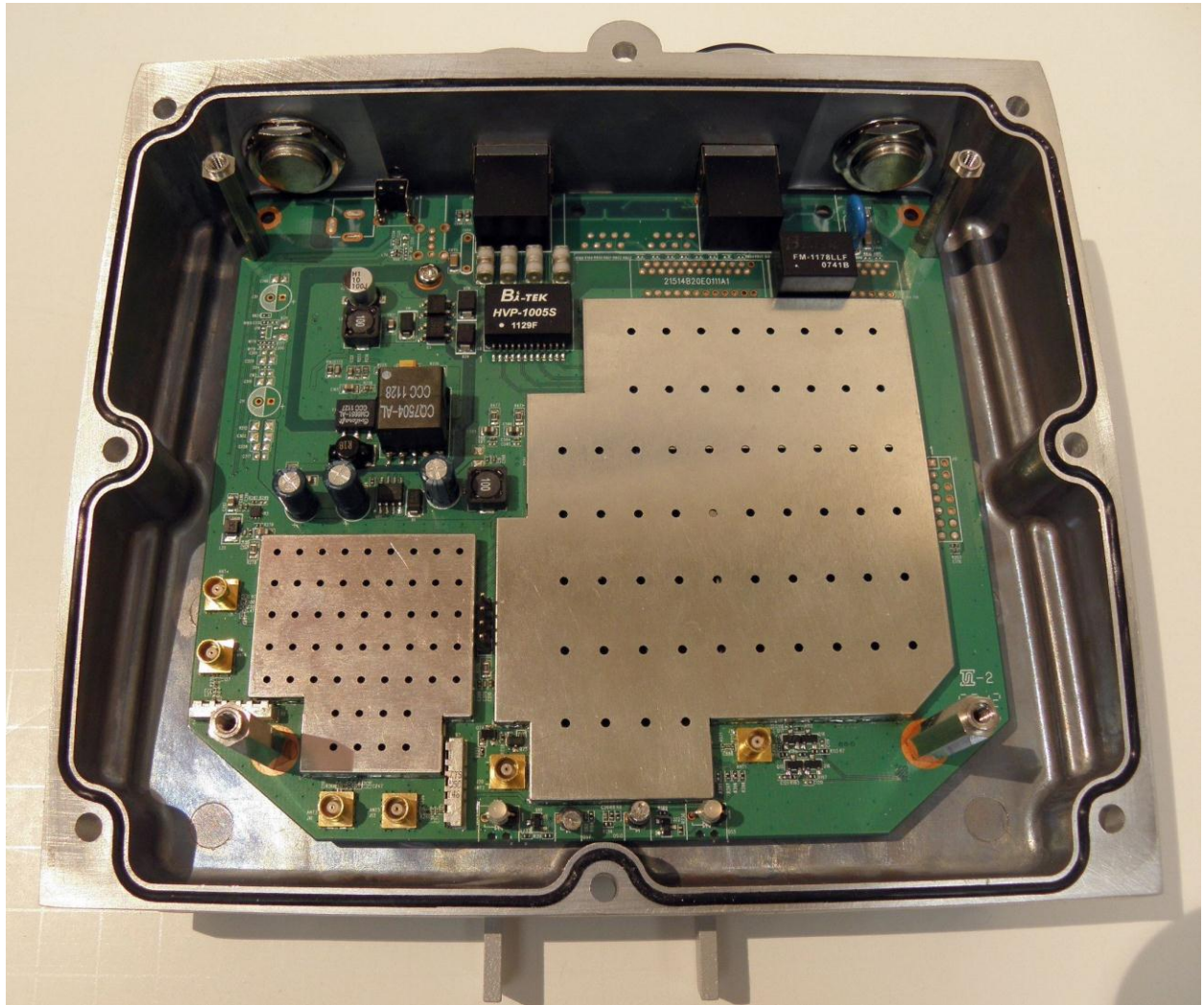
Internal enclosure top
