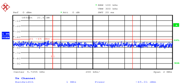
Figure 8.5-66: Upper band edge emission at 5.725 GHz on high channel, 802.11n HT20, ch1
