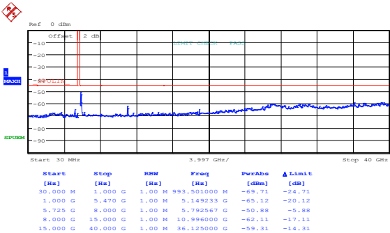
Figure 8.5-31: Peak spurious emissions outside restricted bands at low channel, 802.11a, cho
