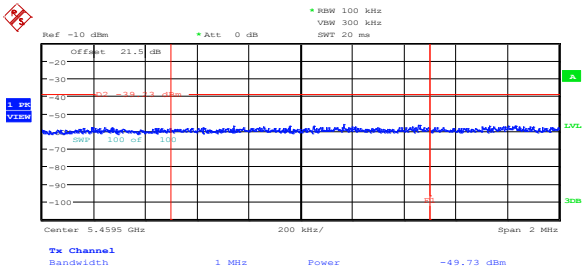
Figure 8.5-2: Peak spurious emission at 5.46 GHz on low channel, 802.11a, cho
