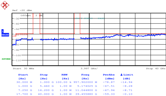
Figure 8.5-13: Peak spurious emissions within restricted bands at low channel, 802.11n HT40, cho
