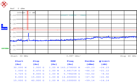
Figure 8.5-41: Peak spurious emissions outside restricted bands at low channel, 802.11n HT40, ch1
