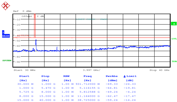
Figure 8.5-47: Peak spurious emissions outside restricted bands at mid channel, 802.11n HT20, cho
