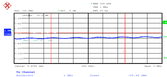
Figure 8.5-18: Average spurious emission at 5.46 GHz on low channel, 802.11n HT40, ch1
