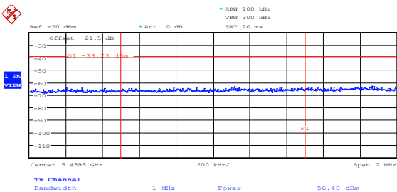
Figure 8.5-17: Peak spurious emission at 5.46 GHz on low channel, 802.11n HT40, ch1
