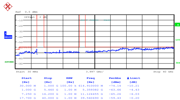
Figure 8.5-24: Peak spurious emissions within restricted bands at mid channel, 802.11n HT40, ch1
