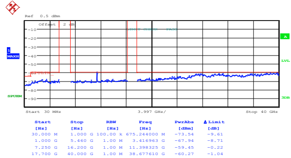
Figure 8.5-26: Peak spurious emissions within restricted bands at high channel, 802.11a, ch1
