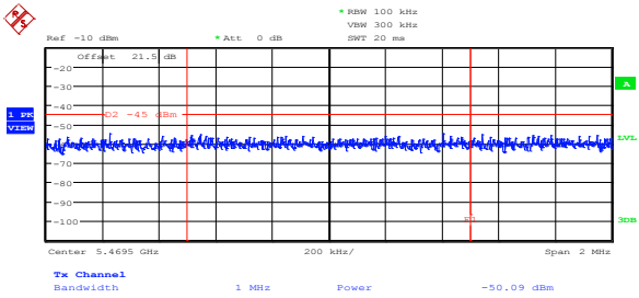
Figure 8.5-32: Lower band edge emission at 5.47 GHz on low channel, 802.11a, cho
