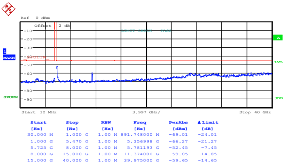
Figure 8.5-70: Peak spurious emissions outside restricted bands at high channel, 802.11n HT40, ch1
