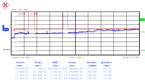
Figure 8.5-23: Peak spurious emissions within restricted bands at mid channel, 802.11n HT40, cho
