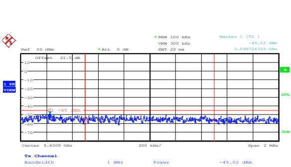
Figure 8.5-48: Upper band edge emission of the first frequency block at 5.6 GHz on mid channel, 802.11n HT20, cho
