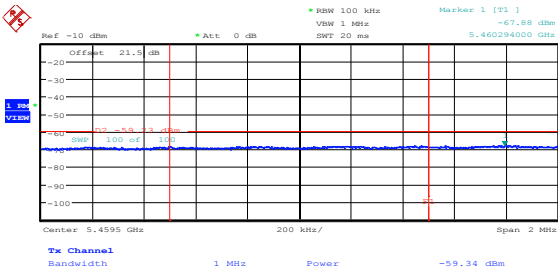
Figure 8.5-3: Average spurious emission at 5.46 GHz on low channel, 802.11a, cho
