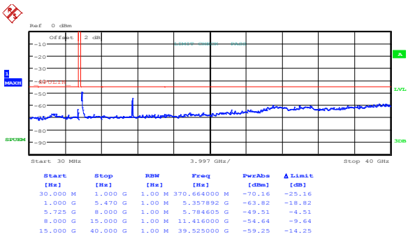
Figure 8.5-58: Peak spurious emissions outside restricted bands at high channel, 802.11a, ch1
