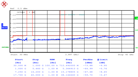
Figure 8.5-10: Peak spurious emissions within restricted bands at low channel, 802.11n HT20, ch1
