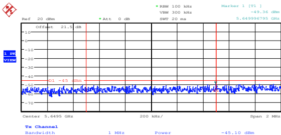
Figure 8.5-59: Lower band edge emission of the second frequency block at 5.65 GHz, 802.11a, ch1
