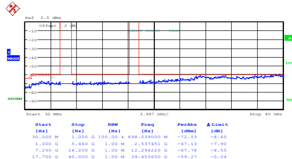
Figure 8.5-16: Peak spurious emissions within restricted bands at low channel, 802.11n HT40, ch1
