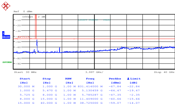
Figure 8.5-55: Peak spurious emissions outside restricted bands at high channel, 802.11a, cho
