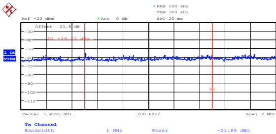
Figure 8.5-11: Peak spurious emission at 5.46 GHz on low channel, 802.11n HT20, ch1
