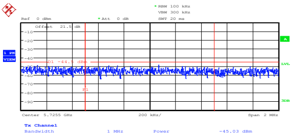
Figure 8.5-72: Upper band edge emission at 5.725 GHz on high channel, 802.11n HT40, ch1
