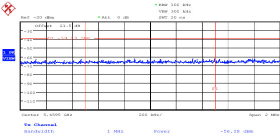
Figure 8.5-5: Peak spurious emission at 5.46 GHz on low channel, 802.11a, ch1
