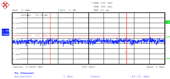
Figure 8.5-42: Lower band edge emission at 5.47 GHz on low channel, 802.11n HT40, ch1
