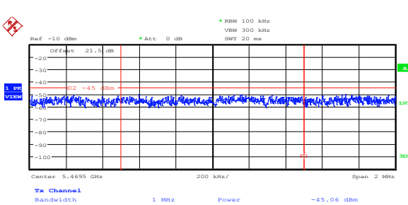
Figure 8.5-40: Lower band edge emission at 5.47 GHz on low channel, 802.11n HT40, cho
