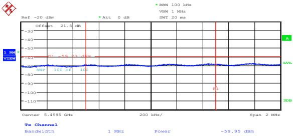
Figure 8.5-6: Average spurious emission at 5.46 GHz on low channel, 802.11a, ch1
