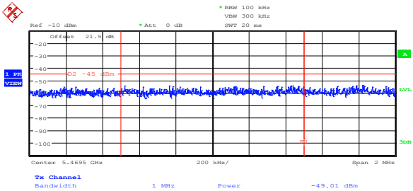
Figure 8.5-36: Lower band edge emission at 5.47 GHz on low channel, 802.11n HT20, cho
