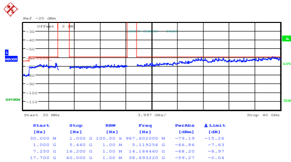
Figure 8.5-29: Peak spurious emissions within restricted bands at high channel, 802.11n HT40, cho
