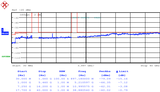
Figure 8.5-1: Peak spurious emissions within restricted bands at low channel, 802.11a, cho
