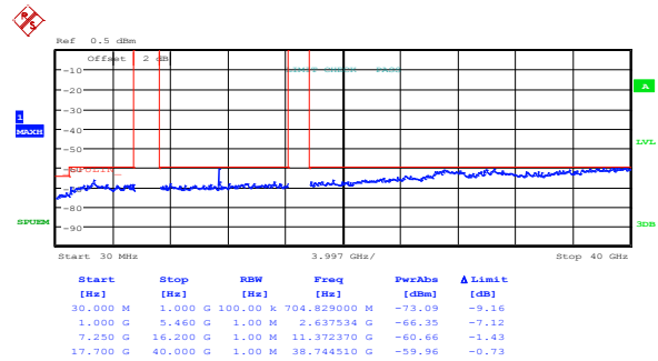
Figure 8.5-30: Peak spurious emissions within restricted bands at high channel, 802.11n HT40, ch1
