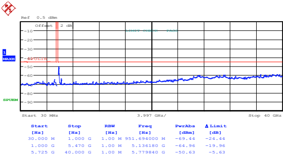
Figure 8.5-39: Peak spurious emissions outside restricted bands at low channel, 802.11n HT40, cho
