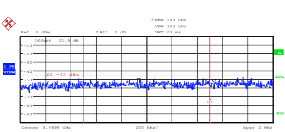
Figure 8.5-34: Lower band edge emission at 5.47 GHz on low channel, 802.11a, ch1
