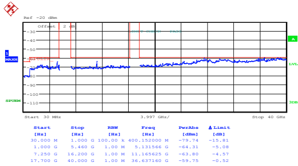
Figure 8.5-19: Peak spurious emissions within restricted bands at mid channel, 802.11a, cho
