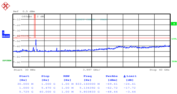
Figure 8.5-51: Peak spurious emissions outside restricted bands at mid channel, 802.11n HT40, cho
