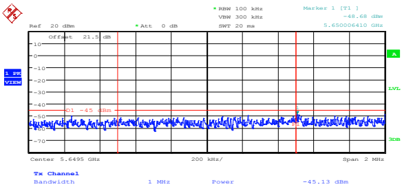
Figure 8.5-62: Lower band edge emission of the second frequency block at 5.65 GHz, 802.11n HT20, cho
