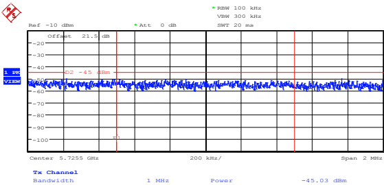
Figure 8.5-69: Upper band edge emission at 5.725 GHz on high channel, 802.11n HT40, cho
