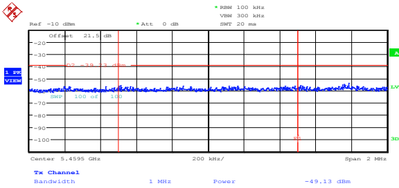
Figure 8.5-8: Peak spurious emission at 5.46 GHz on low channel, 802.11n HT20, cho
