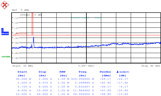
Figure 8.5-37: Peak spurious emissions outside restricted bands at low channel, 802.11n HT20, ch1
