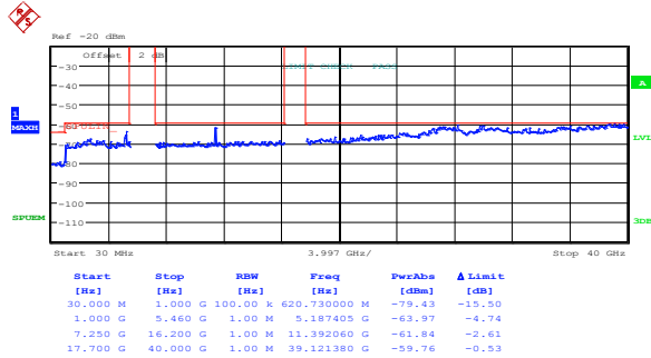
Figure 8.5-25: Peak spurious emissions within restricted bands at high channel, 802.11a, cho
