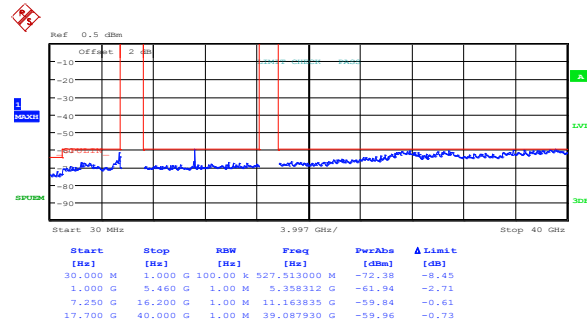
Figure 8.5-20: Peak spurious emissions within restricted bands at mid channel, 802.11a, ch1
