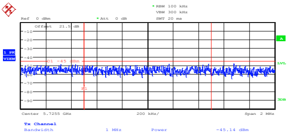
Figure 8.5-60: Upper band edge emission at 5.725 GHz on high channel, 802.11a, ch1
