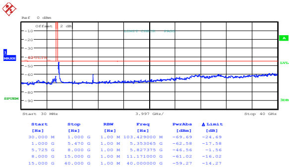
Figure 8.5-45: Peak spurious emissions outside restricted bands at mid channel, 802.11a, ch1
