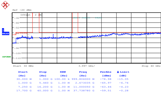
Figure 8.5-7: Peak spurious emissions within restricted bands at low channel, 802.11n HT20, cho
