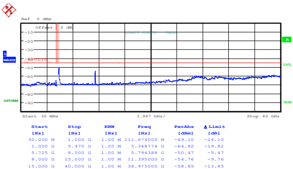
Figure 8.5-64: Peak spurious emissions outside restricted bands at high channel, 802.11n HT20, ch1
