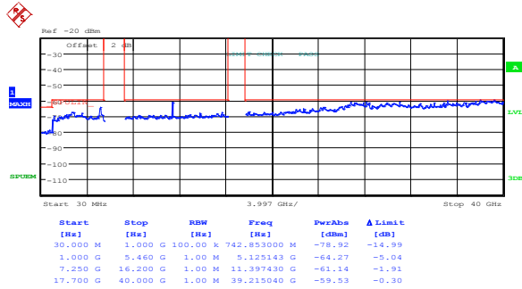
Figure 8.5-27: Peak spurious emissions within restricted bands at high channel, 802.11n HT20, cho
