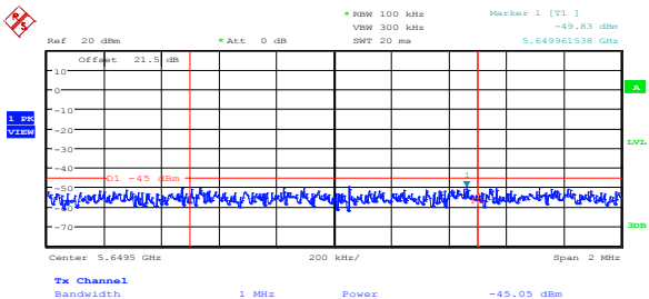
Figure 8.5-68: Lower band edge emission of the second frequency block at 5.65 GHz, 802.11n HT40, cho
