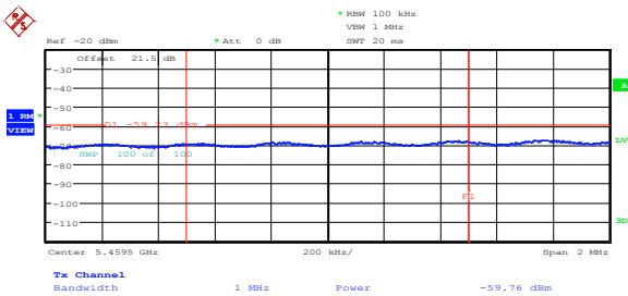
Figure 8.5-12: Average spurious emission at 5.46 GHz on low channel, 802.11n HT20, ch1
