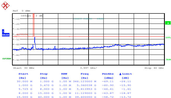
Figure 8.5-53: Peak spurious emissions outside restricted bands at mid channel, 802.11n HT40, ch1
