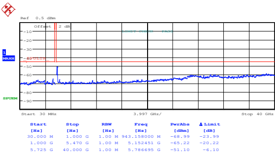
Figure 8.5-67: Peak spurious emissions outside restricted bands at high channel, 802.11n HT40, cho
