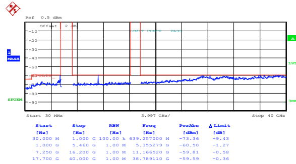
Figure 8.5-22: Peak spurious emissions within restricted bands at mid channel, 802.11n HT20, ch1
