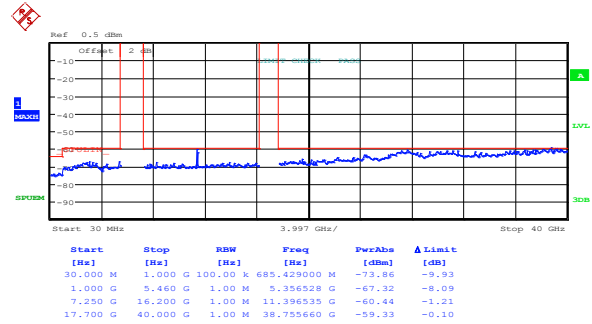
Figure 8.5-28: Peak spurious emissions within restricted bands at high channel, 802.11n HT20, ch1
