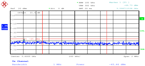
Figure 8.5-44: Upper band edge emission of the first frequency block at 5.6 GHz on mid channel, 802.11a, cho
