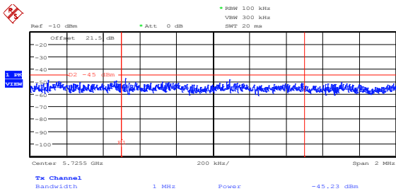
Figure 8.5-57: Upper band edge emission at 5.725 GHz on high channel, 802.11a, cho
