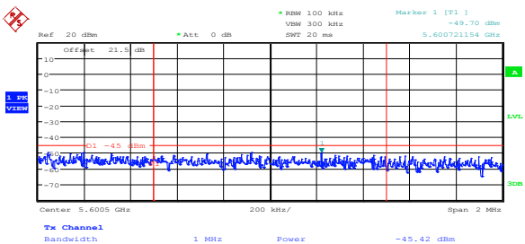
Figure 8.5-52: Upper band edge emission of the first frequency block at 5.6 GHz on mid channel, 802.11n HT40, cho
