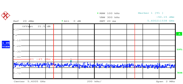
Figure 8.5-46: Upper band edge emission of the first frequency block at 5.6 GHz on mid channel, 802.11a, ch1
