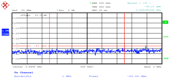
Figure 8.5-56: Lower band edge emission of the second frequency block at 5.65 GHz, 802.11a, cho
