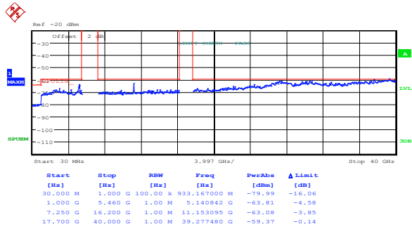
Figure 8.5-21: Peak spurious emissions within restricted bands at mid channel, 802.11n HT20, cho
