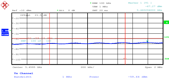
Figure 8.5-15: Average spurious emission at 5.46 GHz on low channel, 802.11n HT40, cho
