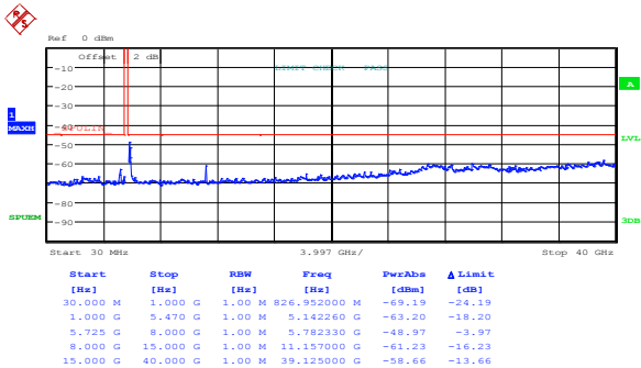
Figure 8.5-43: Peak spurious emissions outside restricted bands at mid channel, 802.11a, cho
