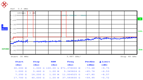
Figure 8.5-4: Peak spurious emissions within restricted bands at low channel, 802.11a, ch1
