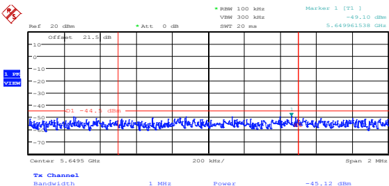
Figure 8.5-71: Lower band edge emission of the second frequency block at 5.65 GHz, 802.11n HT40, ch1
