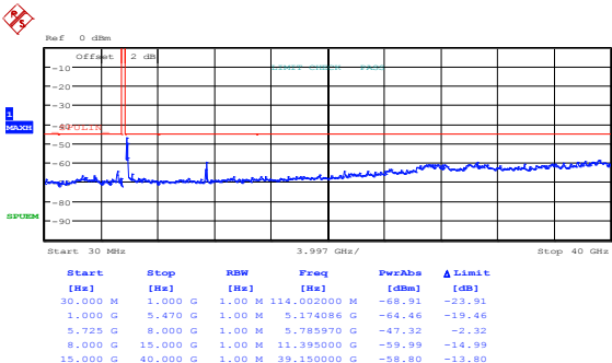
Figure 8.5-61: Peak spurious emissions outside restricted bands at high channel, 802.11n HT20, cho
