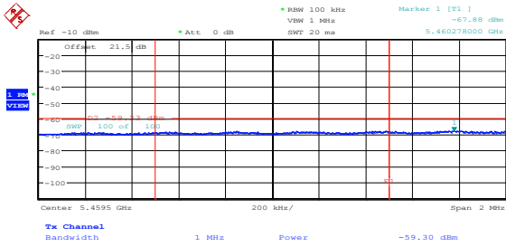
Figure 8.5-9: Average spurious emission at 5.46 GHz on low channel, 802.11n HT20, cho
