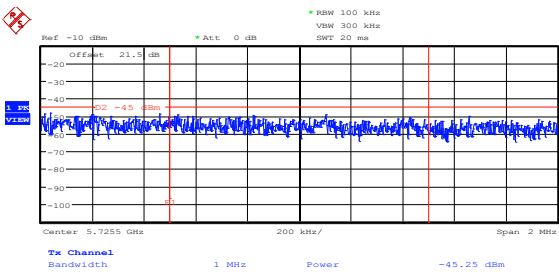
Figure 8.5-63: Upper band edge emission at 5.725 GHz on high channel, 802.11n HT20, cho
