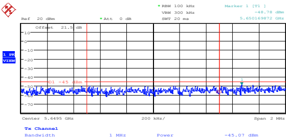
Figure 8.5-65: Lower band edge emission of the second frequency block at 5.65 GHz, 802.11n HT20, ch1
