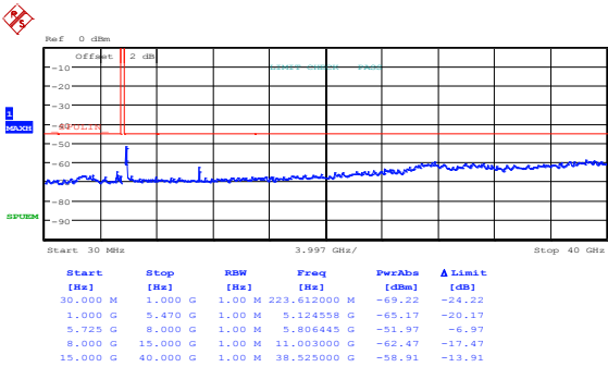
Figure 8.5-35: Peak spurious emissions outside restricted bands at low channel, 802.11n HT20, cho
