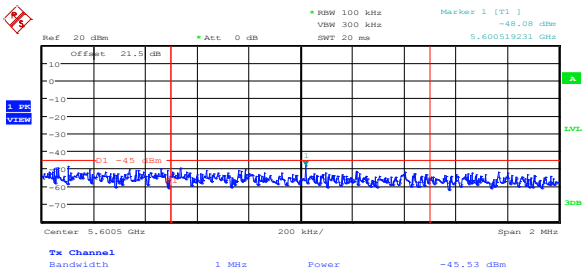
Figure 8.5-50: Upper band edge emission of the first frequency block at 5.6 GHz on mid channel, 802.11n HT20, ch1
