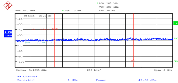
Figure 8.5-14: Peak spurious emission at 5.46 GHz on low channel, 802.11n HT40, cho
