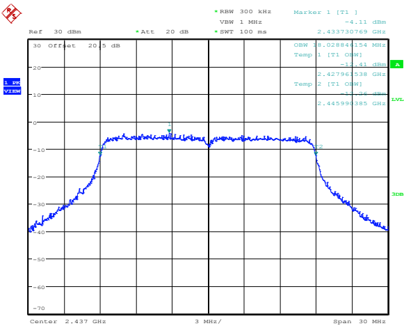
Figure 8.3-1: 99 % bandwidth on 802.11b, sample plot
