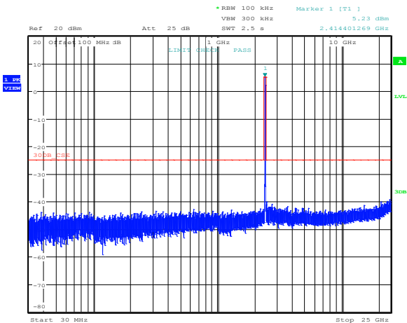
Figure 8.5-13: Conducted spurious emissions for 802.11b, ch1, low channel
