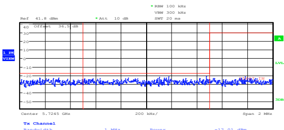
Figure 8.6-71: Lower band edge emission at 5.725 GHz, 802.11n HT40, 11.5 dBi antenna, cho
