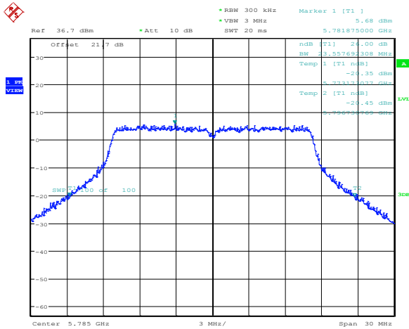
Figure 8.2-1: 26 dB bandwidth on 802.11a, sample plot
