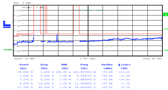
Figure 8.6-40: Peak spurious emissions within restricted bands at FCC high channel, 802.11n HT20, ch1
