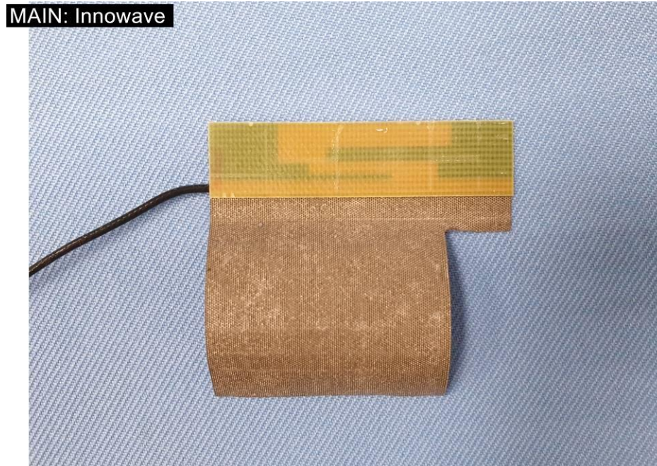
EUT Photo (28)
