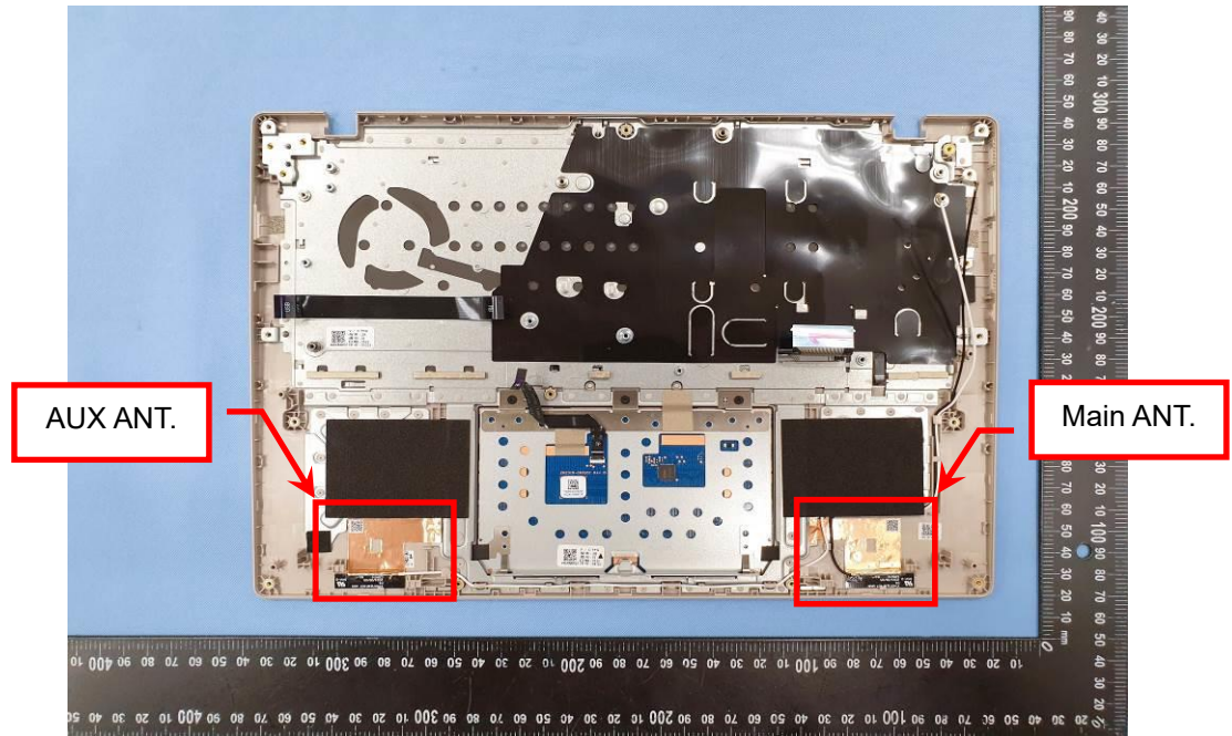
EUT Photo (34)
