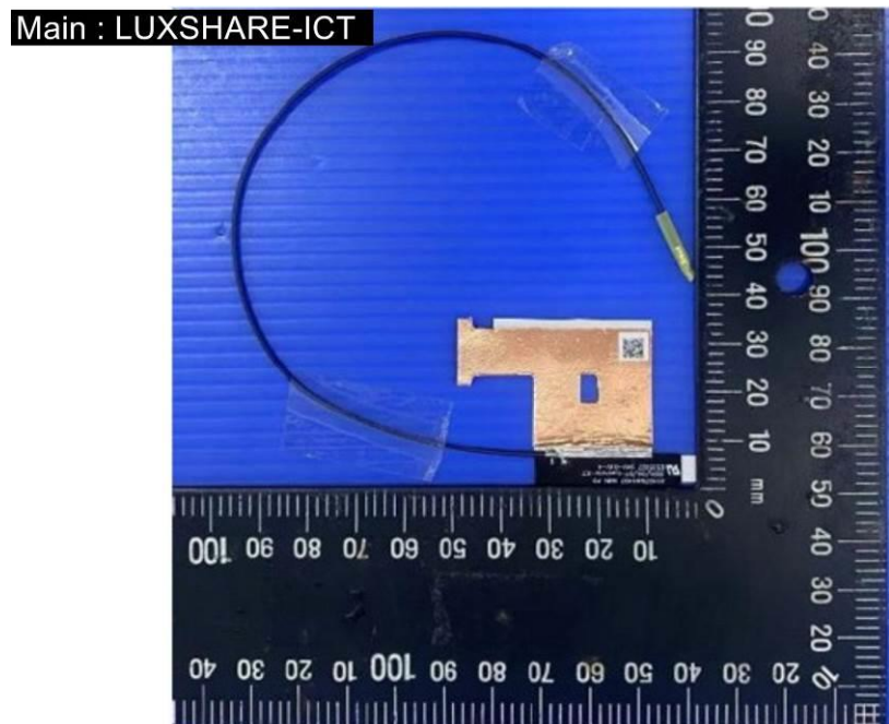
EUT Photo (34)
