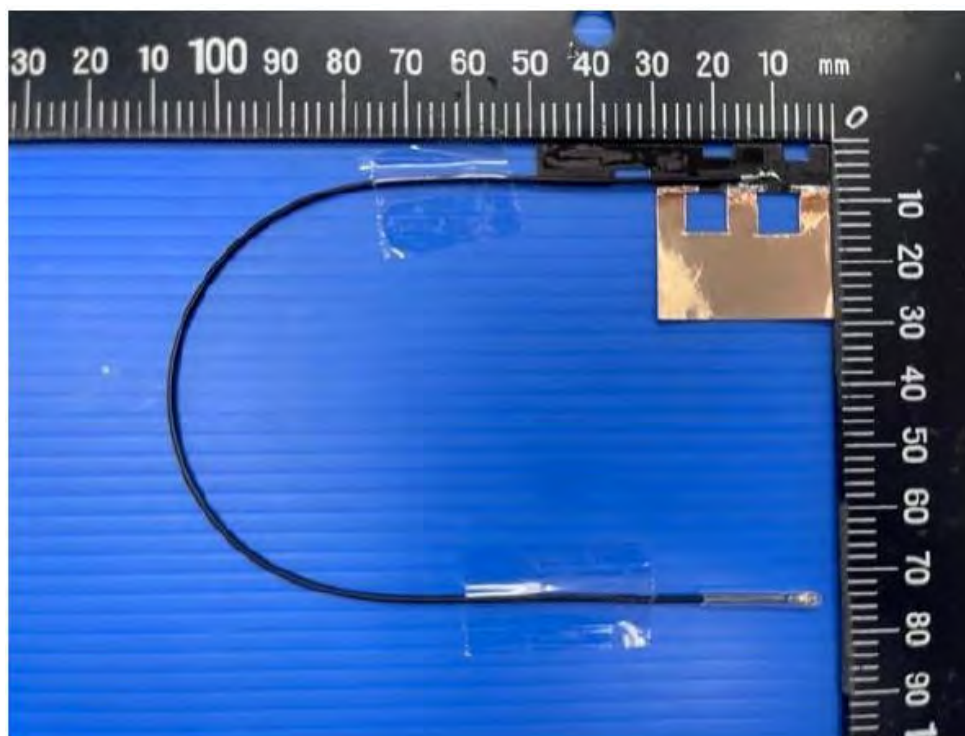
(28) EUT Photo_Pulse Main Antenna
