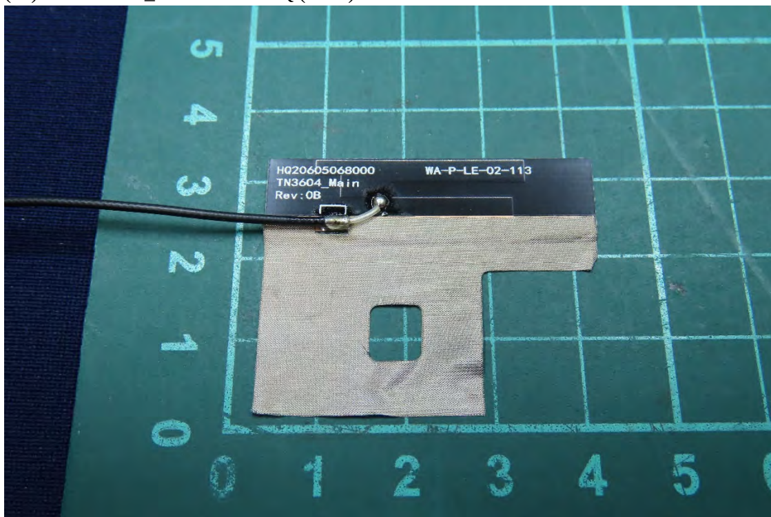
(22) EUT Photo _Antenna: INPAQ (Main)
