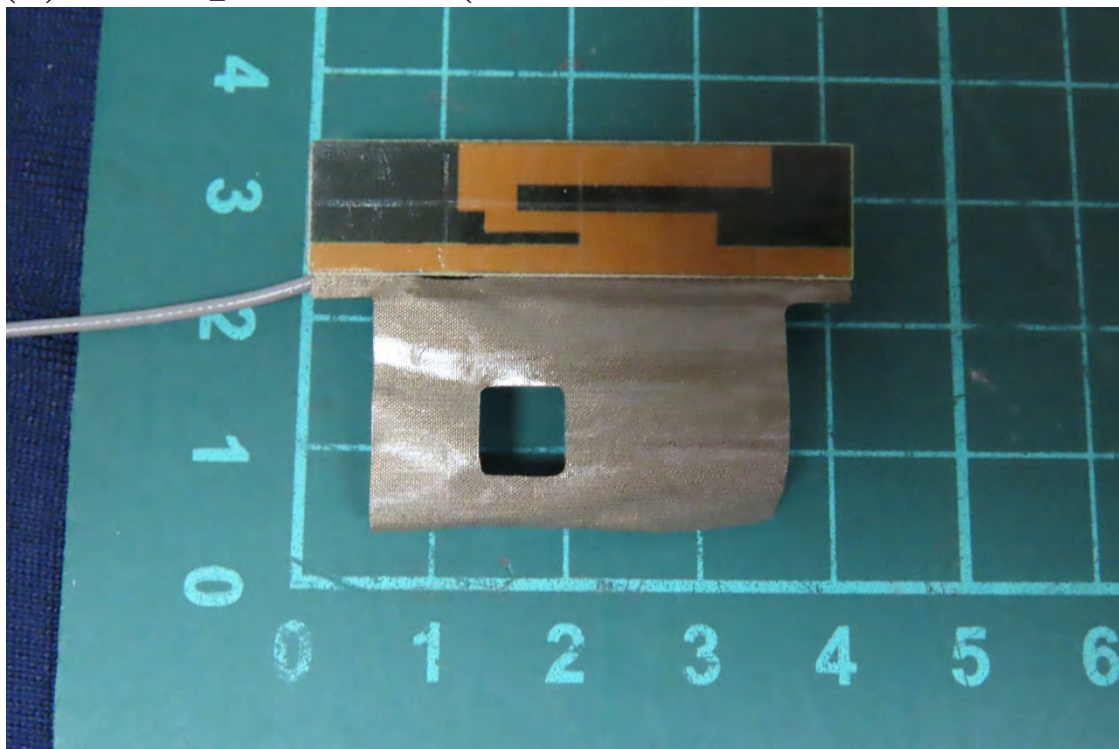
(29) EUT Photo _Antenna: Innowave (Aux
