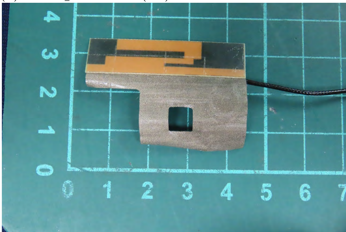
(27) EUT Photo _Antenna: Innowave (Main)
