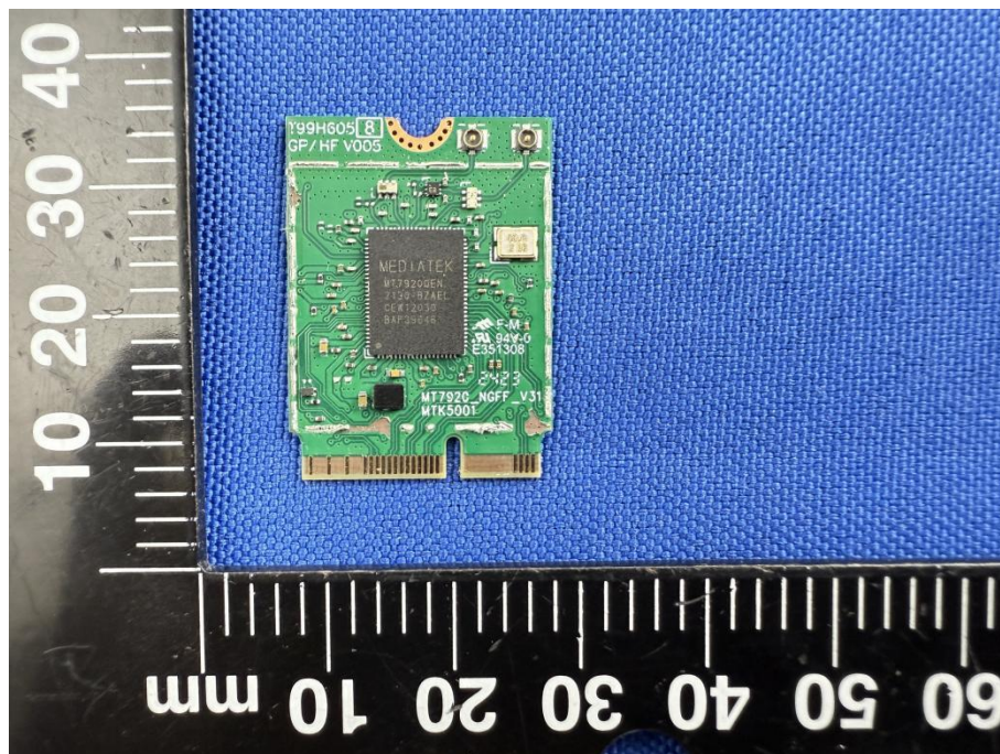
RF MODULE TOP VIEW-MT7920(WITHOUT SHIELDING)
