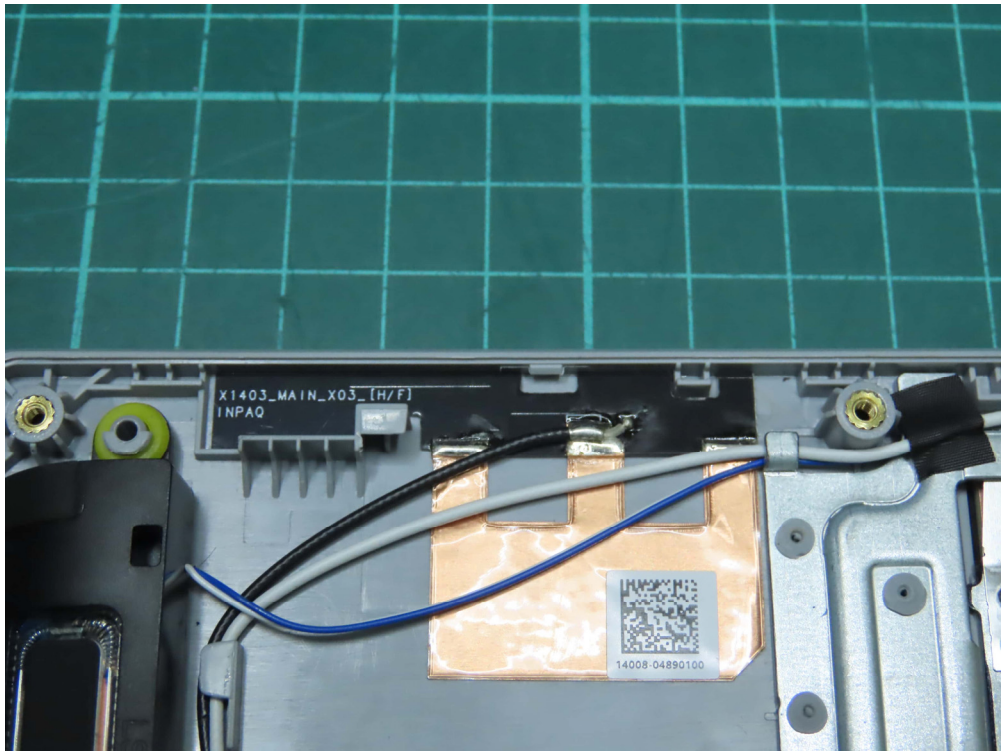
(34) EUT Photo
