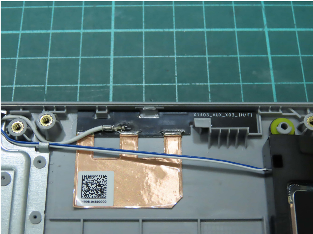
(35) EUT Photo
