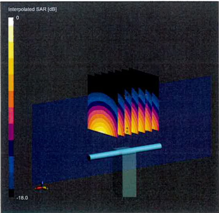
0 dB = 27.5 W/Kg
