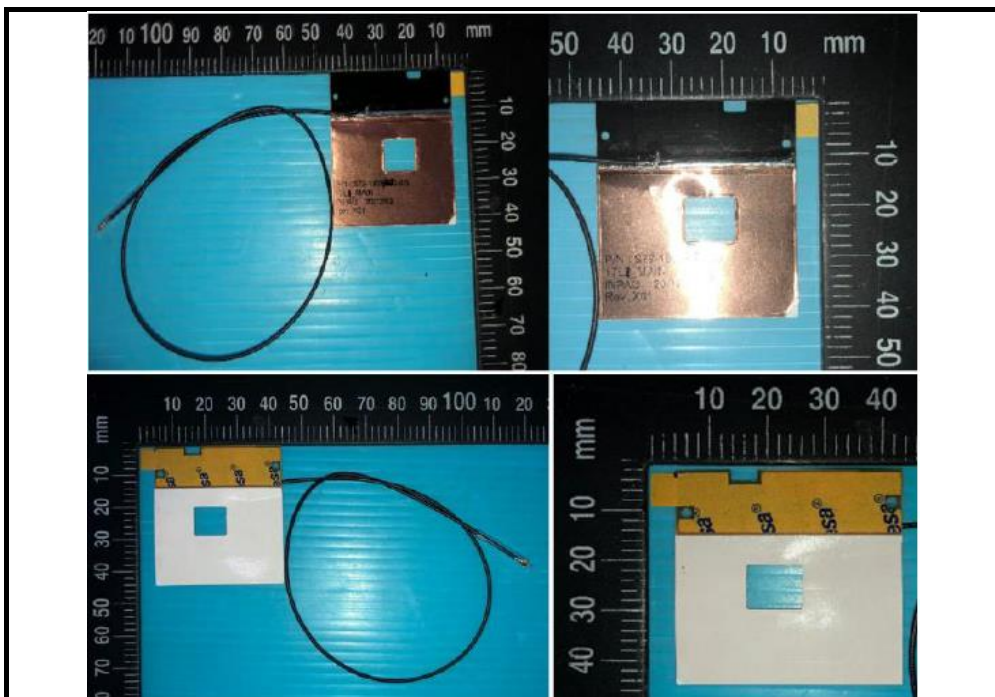
Ant. Set 3 (Brand: MSI / Model: WA-P-LE-02-045)
