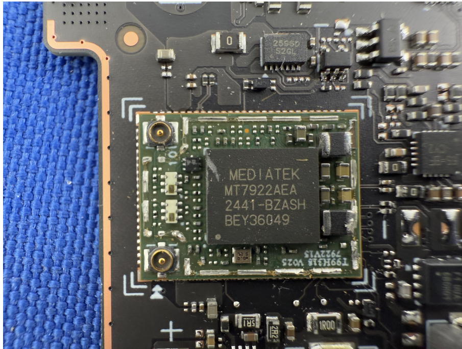
RF MODULE TOP VIEW-MT7922A12L(WITHOUT SHIELDING)
