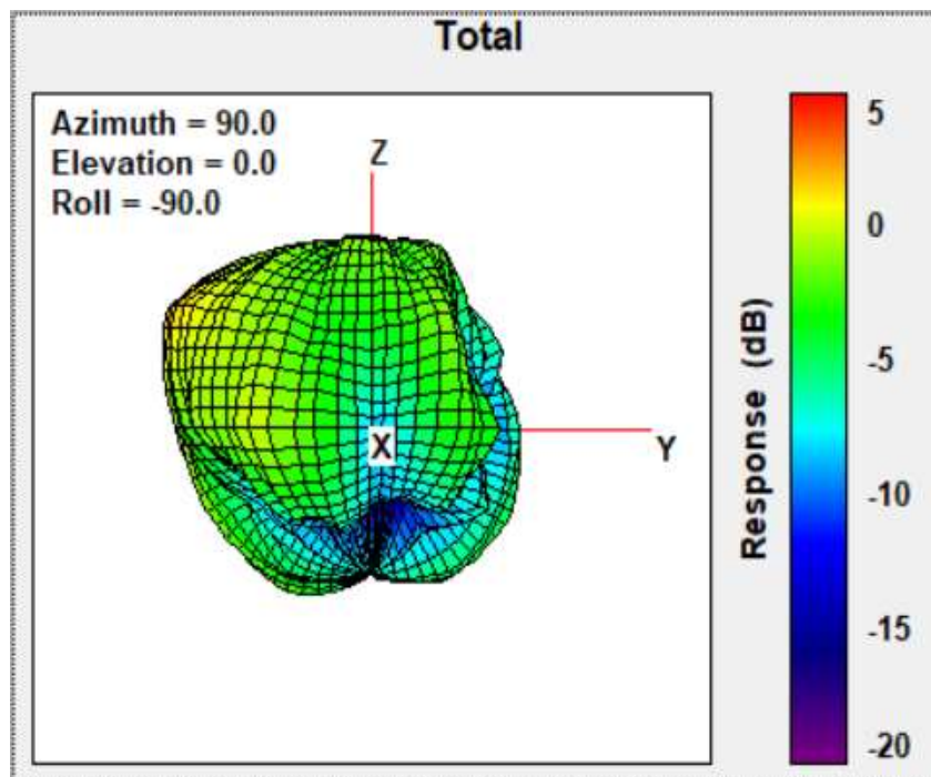
Max Antenna 3D Radiation Pattern 6525-6875 MHz
