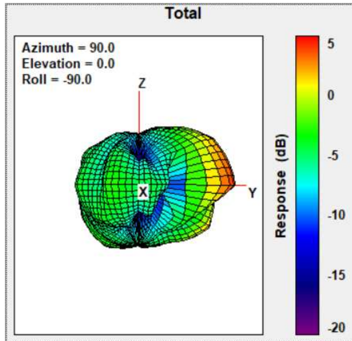
Max Antenna 3D Radiation Pattern 5150-5250 MHz
