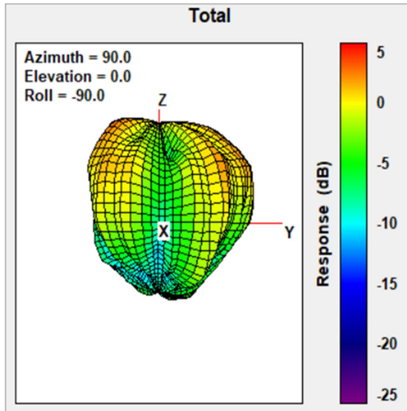
Max Antenna 3D Radiation Pattern 6875-7125 MHz
