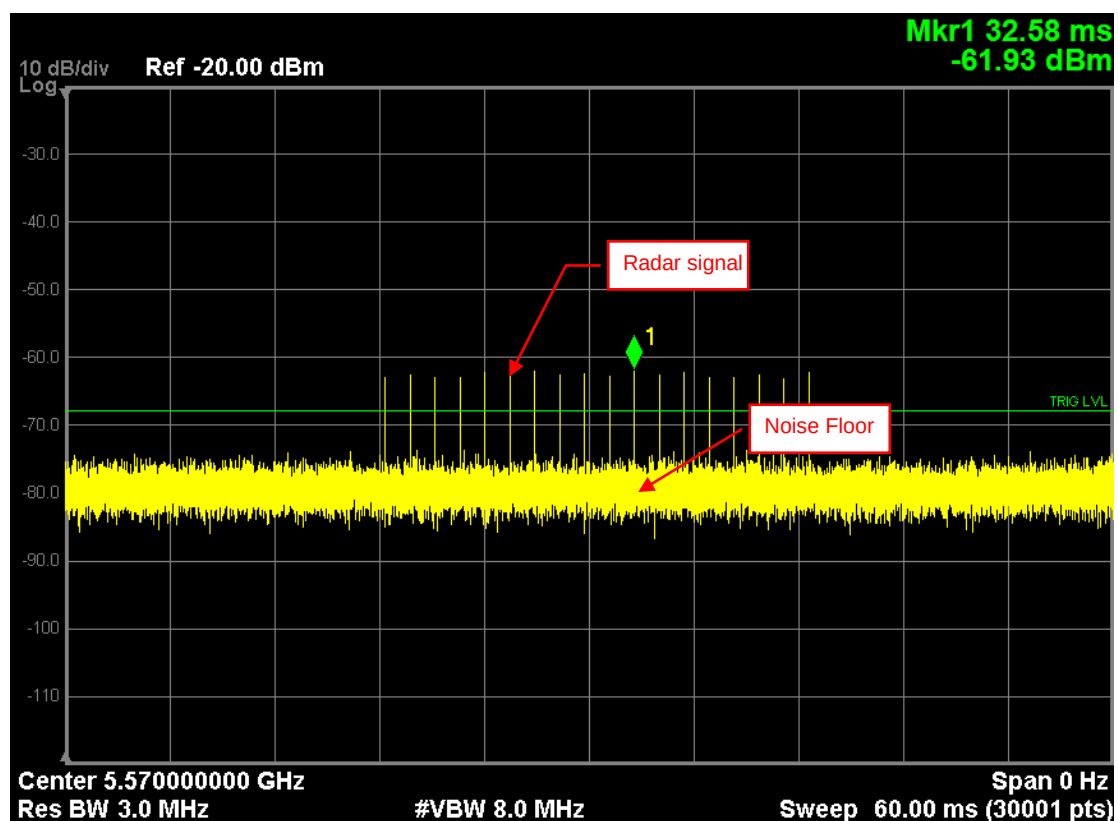
Radar Signal 0
