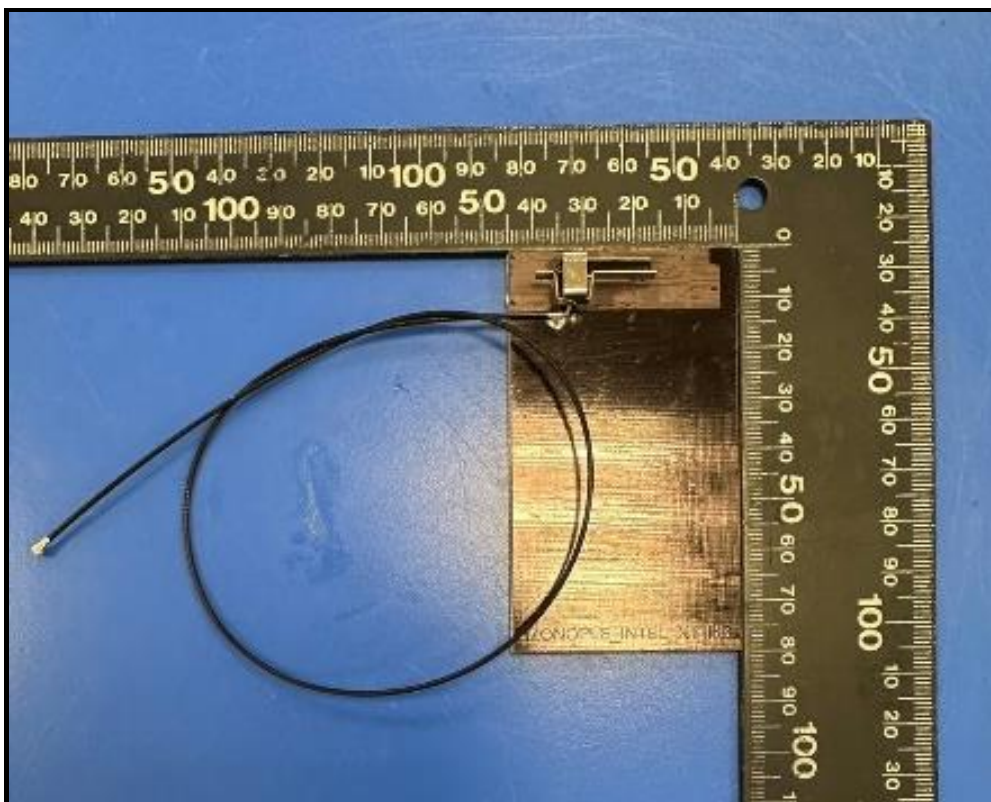
Monopole Antenna (Model: 260-25105)
