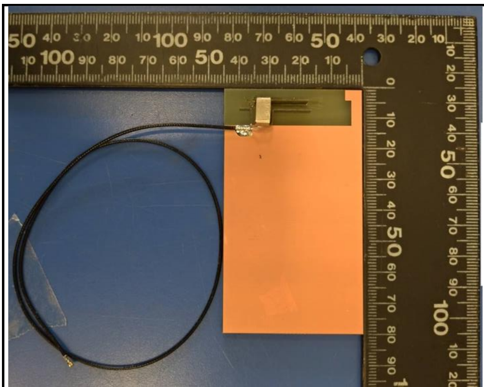
Monopole Antenna (Model: 260-25106)
