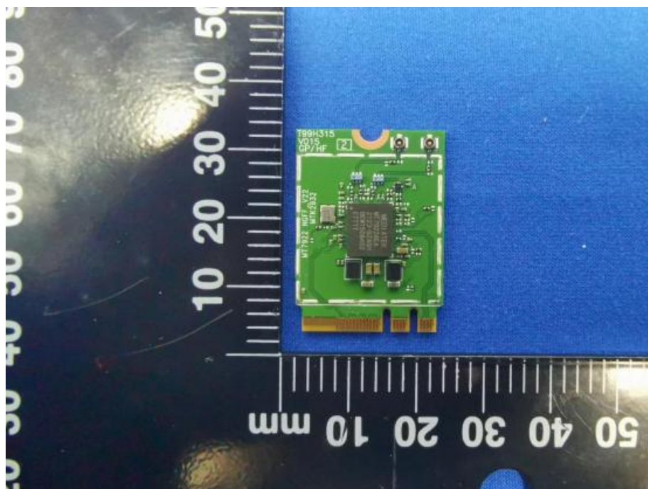
RF MODULE TOP VIEW-MT7922A22M(WITHOUT SHIELDING)
