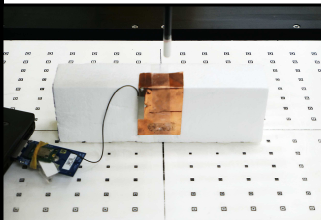
Right Side of EUT Tested at 8 mm
