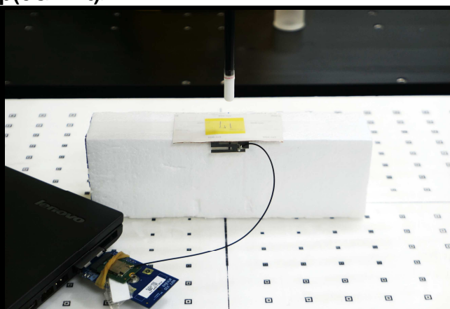
Rear Face of EUT Tested at 8 mm
