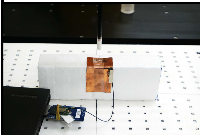
Left Side of EUT Tested at 8 mm
