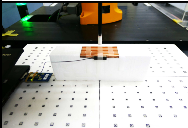
Bottom Side of EUT Tested at 8 mm
