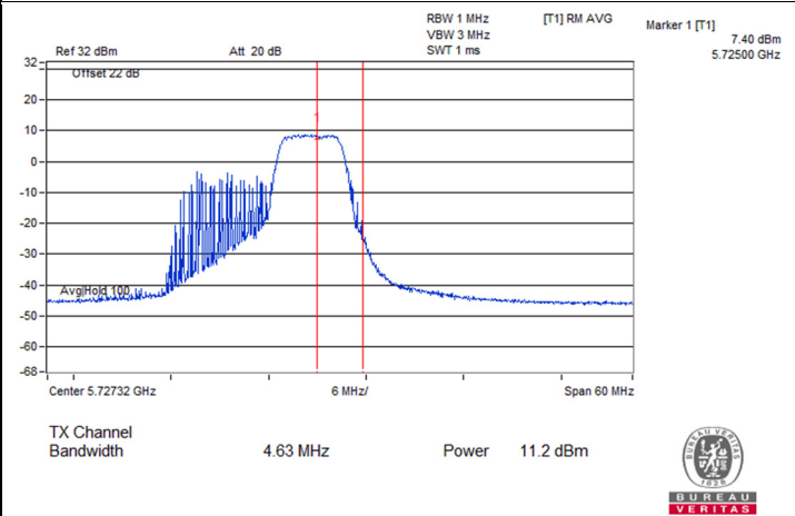
802.11be (EHT20) 52+26-tone MRU 1S1T : CH 144 (U-NII-3)
