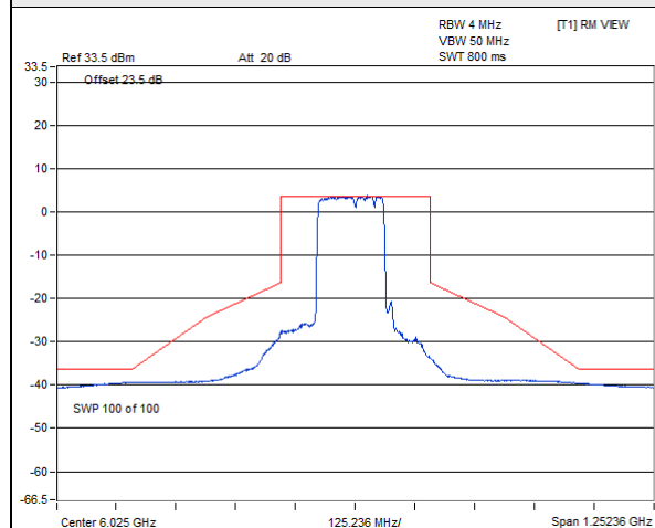
802.11be (EHT160) 996+484+242-tone MRU SP Client_1T1S : CH 15@99_1
