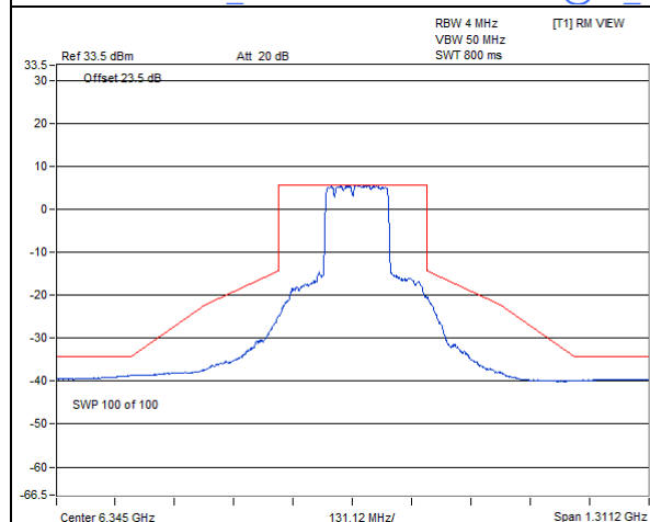
802.11be (EHT160) 996+484+242-tone MRU SP Client_2T2S / Chain 1 : CH 79@96_0
