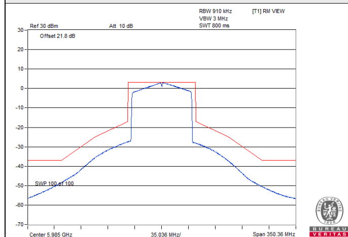
802.11ax (HE80) SP Client 1S1T / Chain 0 : CH 7
