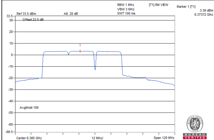
802.11be (EHT80) 484+242-tone MRU SP Client_1T1S : CH 87@90
