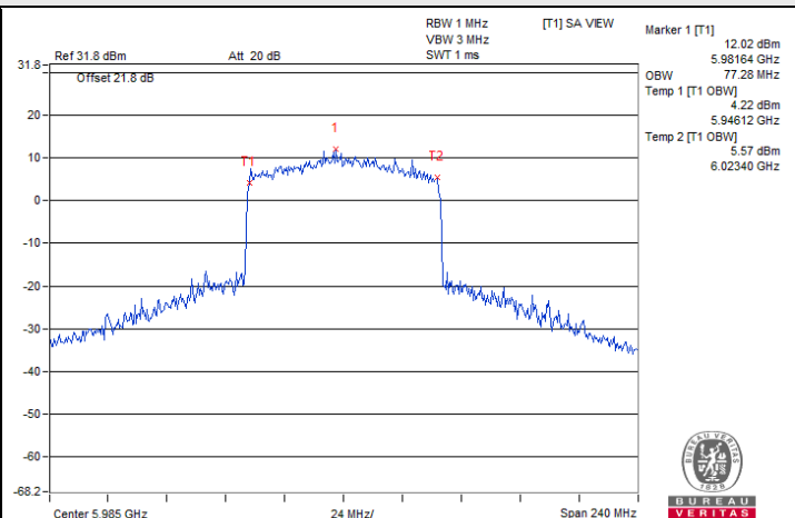
802.11ax (HE80) SP Client 2T2S / Chain 0 : CH 7
