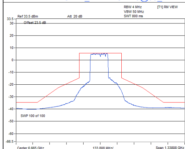
802.11be (EHT160) 996+484+242-tone MRU SP Client_1T1S : CH 143@99_1
