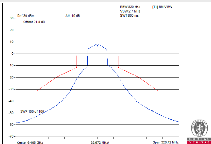
802.11ax (HE40) SP Client 1S1T / Chain 0 : CH 91
