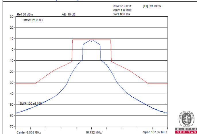
802.11ax (HE20) SP Client 1S1T / Chain 0 : CH 117
