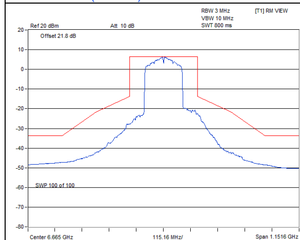
802.11ax (HE160) SP Client 1S1T / Chain 0 : CH 143
