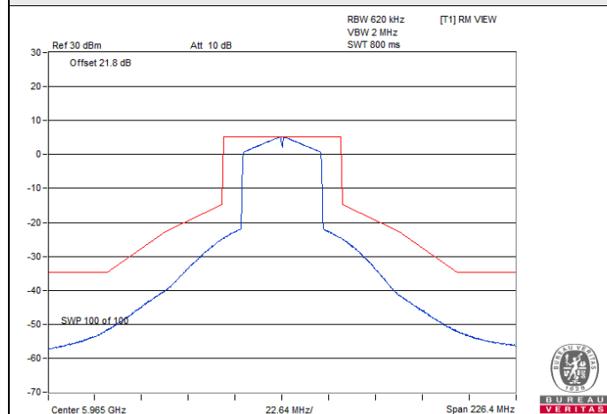
802.11ax (HE40) SP Client 1S1T / Chain 0 : CH 3
