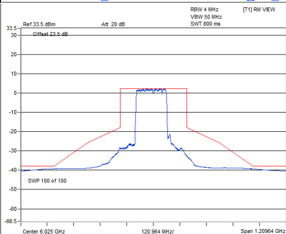
802.11be (EHT160) 996+484+242-tone MRU SP Client_2T2S / Chain 1 : CH 15@99_1
