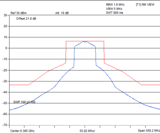
802.11ax (HE80) SP Client 2S2T / Chain 1 : CH 87
