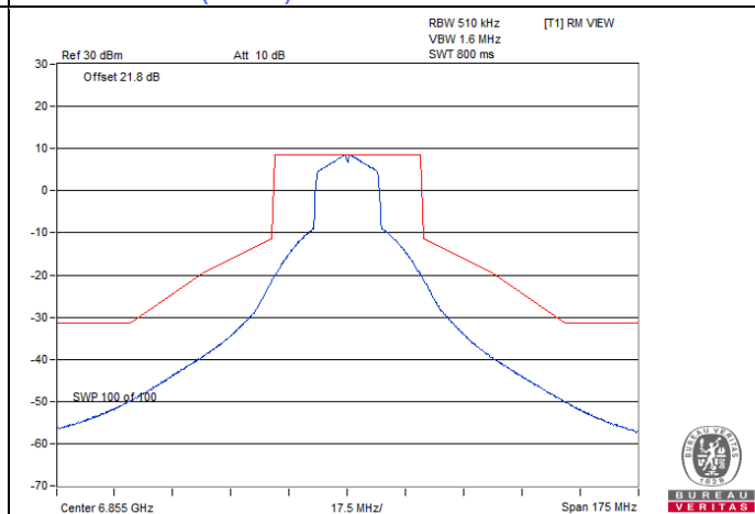
802.11ax (HE20) SP Client 1S1T / Chain 0 : CH 181
