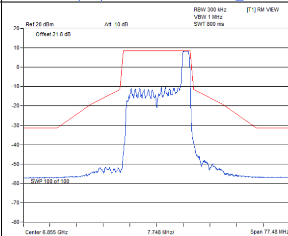
802.11ax (HE) 26-tone RU SP Client_1T1S : CH 181@8
