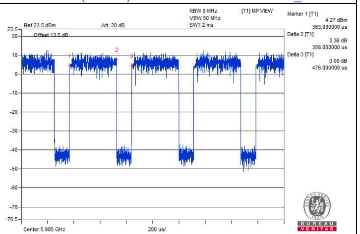
802.11be (EHT80) 484+242-tone MRU SP Client_1T1S
