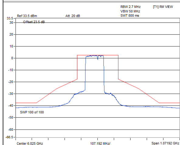
802.11be (EHT160) 996+484-tone MRU SP Client_1T1S : CH 15@95_1
