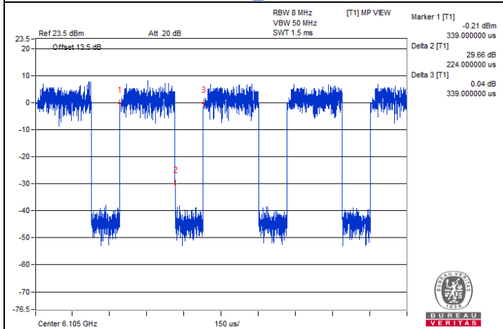
802.11be (EHT320) 3x996-tone MRU SP Client 2T2S
