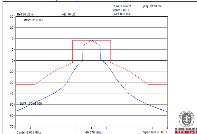
802.11ax (HE80) SP Client 1S1T / Chain 0 : CH 135
