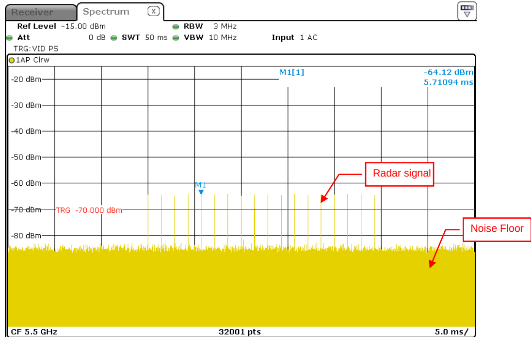
Radar Signal 0
