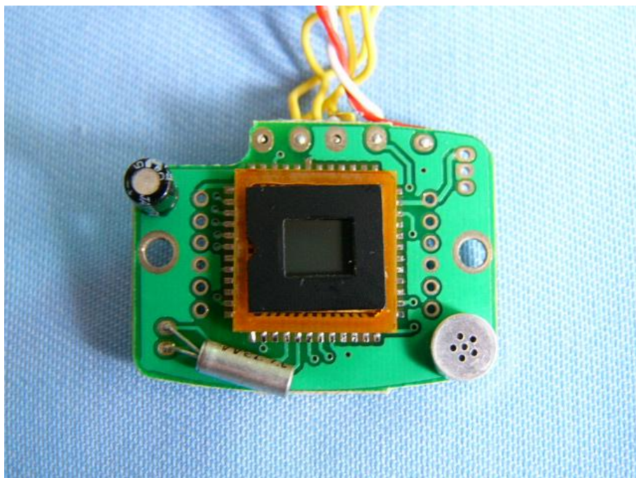
(4) Main&RF board component side
