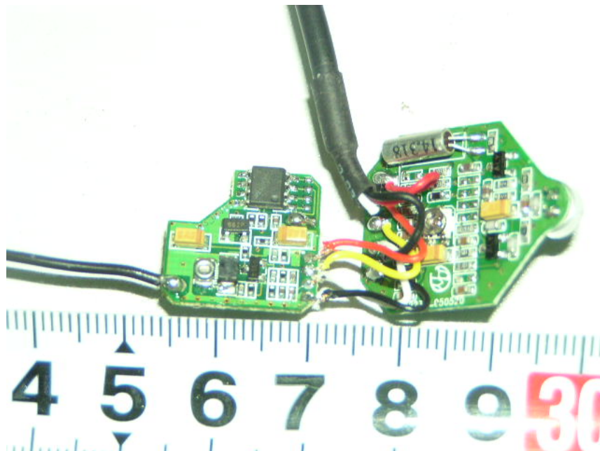
EUT-PCB View (3)
