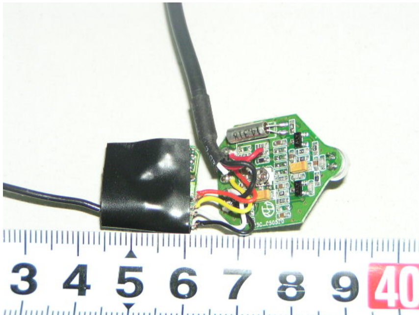
EUT-PCB View (1)
