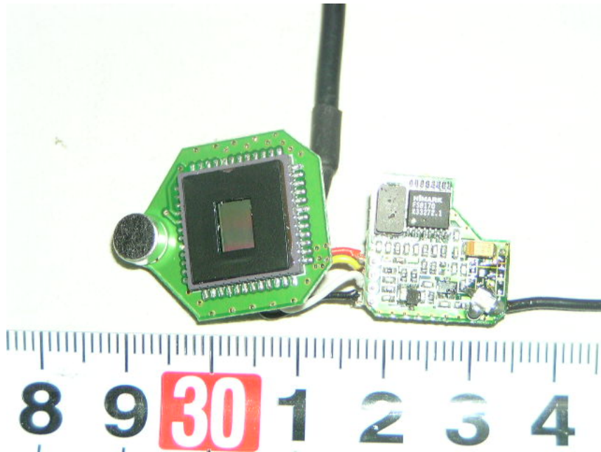
EUT-PCB View (2)
