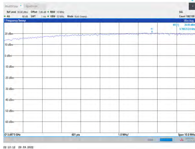
Band48-5MHz-16QAM-56715-1RB#24
