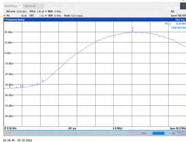
Band48-20MHz-16QAM-55340-1RB#99
