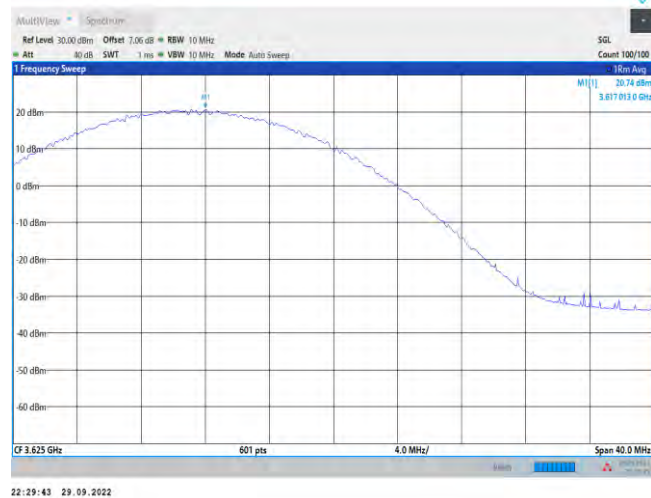
Band48-20MHz-QPSK-55990-1RB#0
