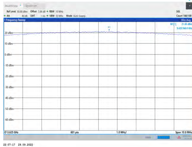
Band48-5MHz-QPSK-55990-1RB#24
