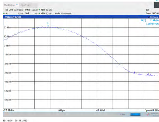
Band48-20MHz-16QAM-56640-1RB#0
