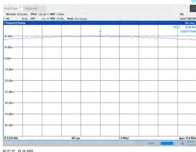
Band48-5MHz-16QAM-55990-1RB#12
