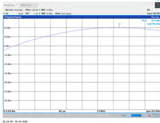
Band48-10MHz-QPSK-55990-1RB#49
