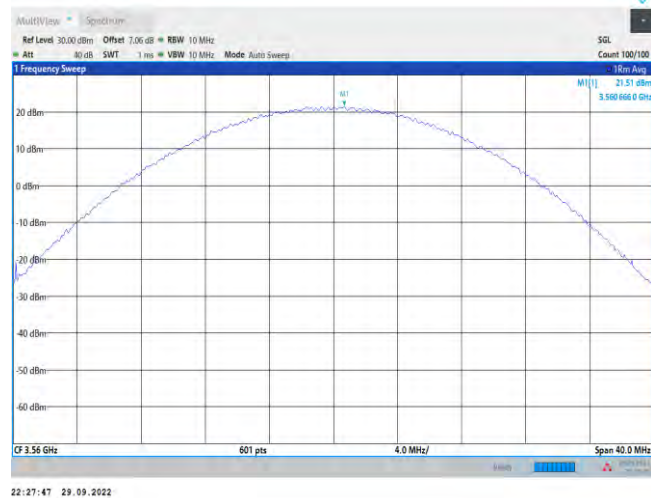
Band48-20MHz-QPSK-55340-1RB#49
