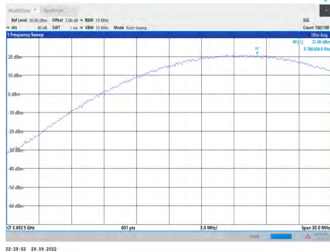
Band48-15MHz-16QAM-56665-1RB#74
