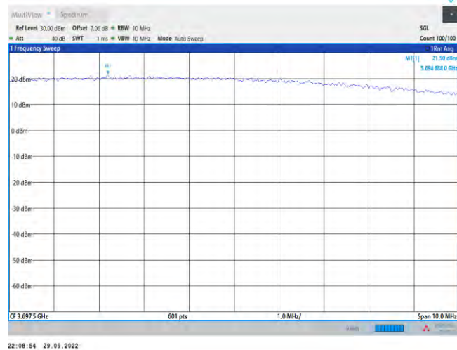
Band48-5MHz-16QAM-56715-1RB#0
