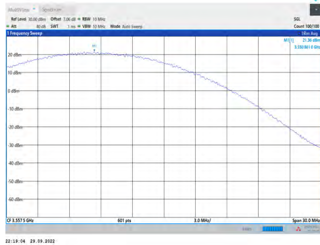
Band48-15MHz-QPSK-55315-1RB#38
