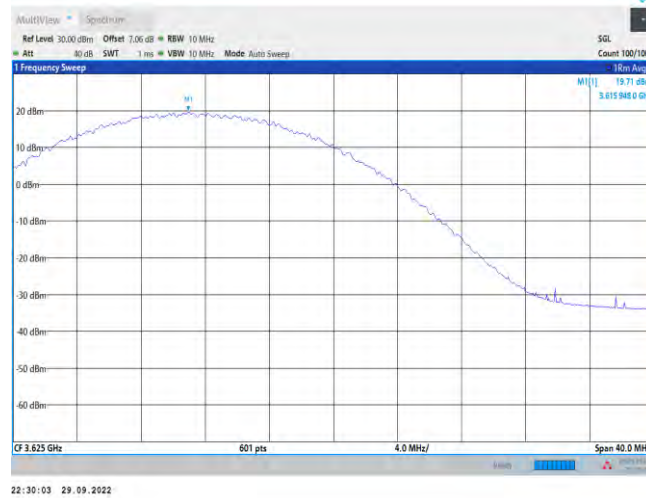
Band48-20MHz-16QAM-55990-1RB#49
