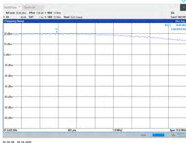
Band48-5MHz-16QAM-55990-1RB#12
