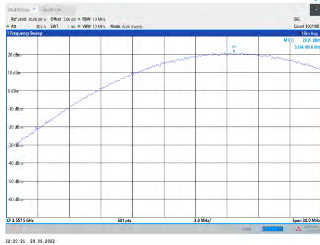
Band48-15MHz-QPSK-55990-1RB#0
