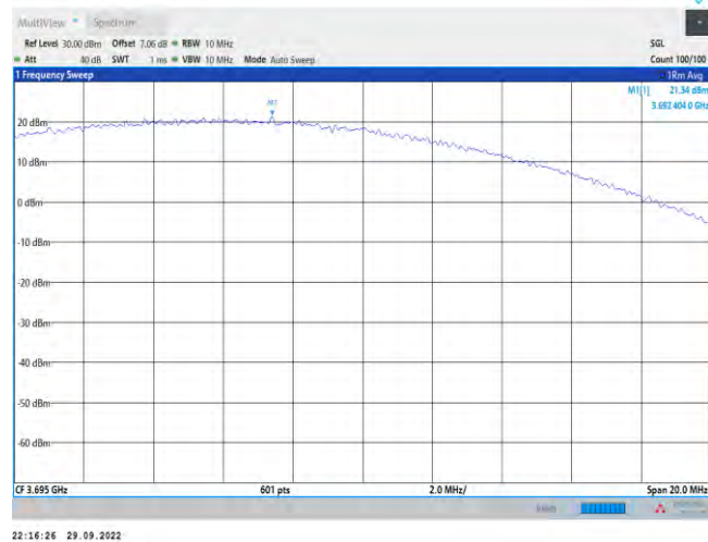
Band48-10MHz-16QAM-56690-1RB#0
