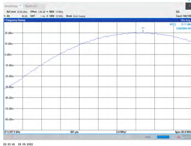
Band48-15MHz-16QAM-55315-1RB#74
