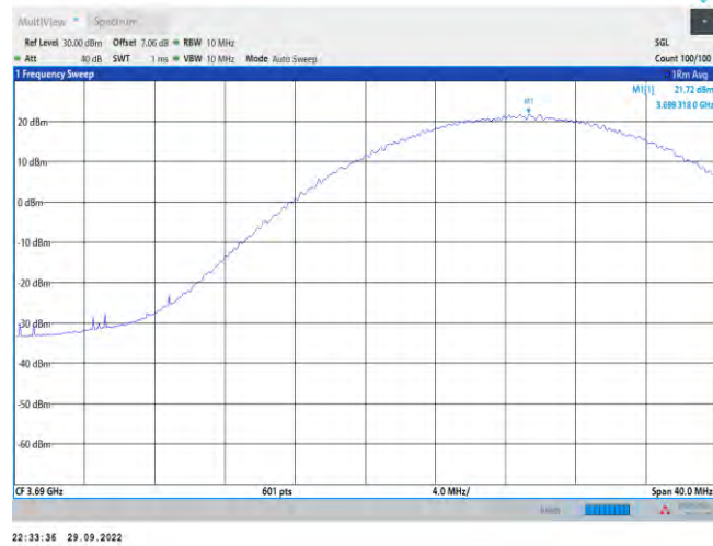
Band48-20MHz-16QAM-55340-1RB#0
