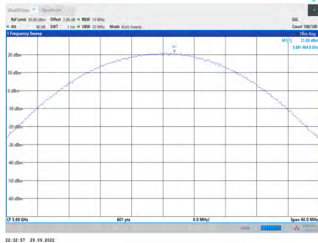
Band48-20MHz-QPSK-56640-1RB#49
