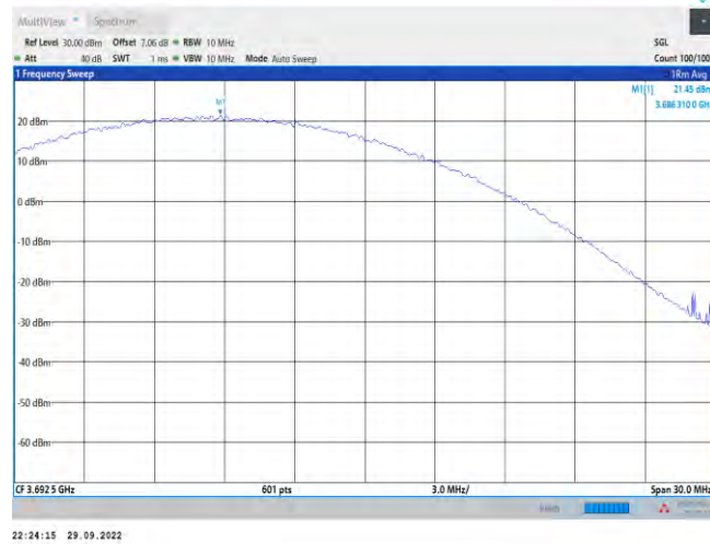
Band48-15MHz-QPSK-56665-1RB#38
