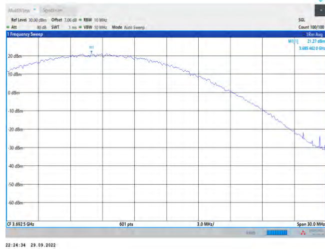
Band48-15MHz-16QAM-56665-1RB#0
