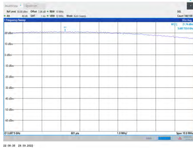
Band48-5MHz-QPSK-56715-1RB#12
