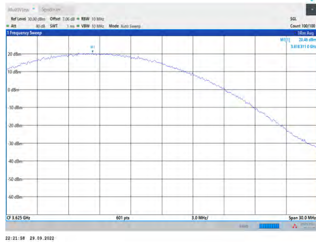
Band48-15MHz-16QAM-55990-1RB#38
