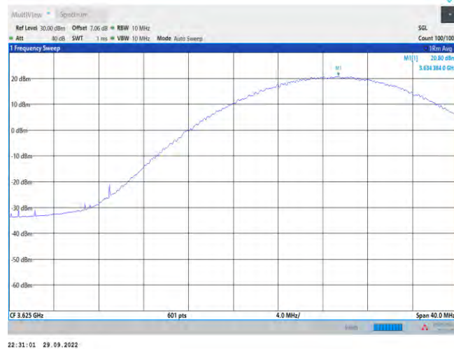
Band48-20MHz-QPSK-55990-1RB#99
