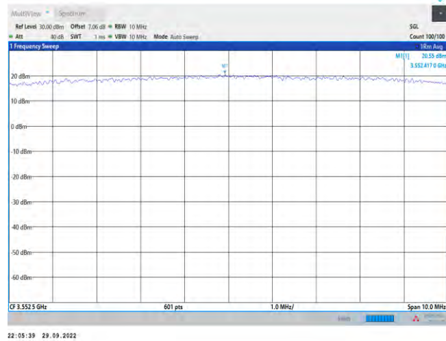
Band48-5MHz-16QAM-55265-1RB#24
