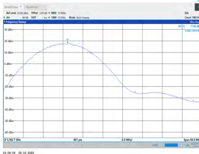
48-48-10MHz-20MHz-QPSK-QPSK-55295-55439-50RB#0-100RB#0
