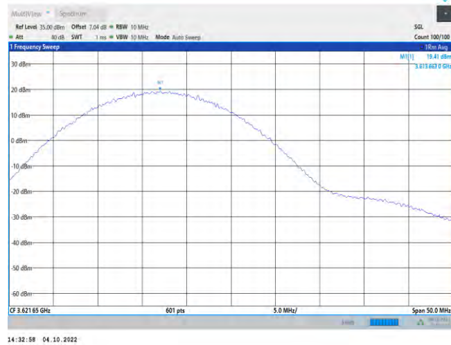
48-48-5MHz-20MHz-QPSK-QPSK-55898-56015-25RB#0-100RB#0
