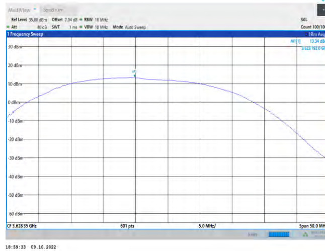
48-48-20MHz-5MHz-QPSK-QPSK-55965-56082-1RB#0-0RB#0
