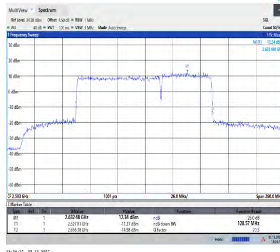
1-41-41-80+50-M-4-DFT-16QAM-Outet_Full
