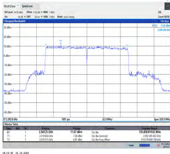
1-41-41-80+80-M-1-DFT-QPSK-Outer_Full
