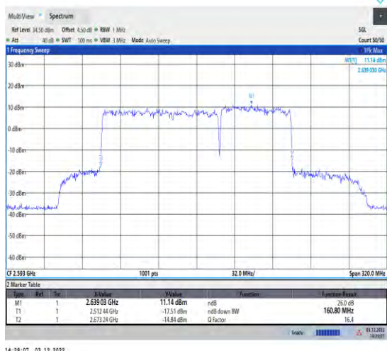
1-41-41-100+60-M-3-DFT-16QAM-Outer_Full
