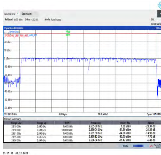
1-41-41-30-80+80-H-3-DFT-QPSK-Outer_Full
