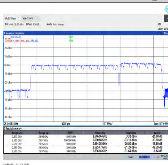
1-41-41-30-100+50-H-3-DFT-QPSK-Outer_Full
