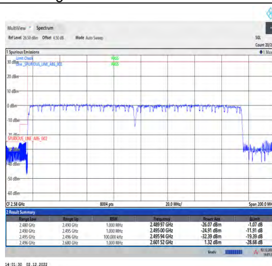
1-41-41-30-80+80-L-6-CP-QPSK-Outer_Full
