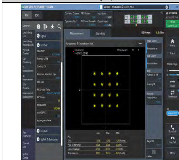
1-41-41-30-100-M-7-CP-16QAM-Outer_Full-273@0-Ant1-see graph-PASS
