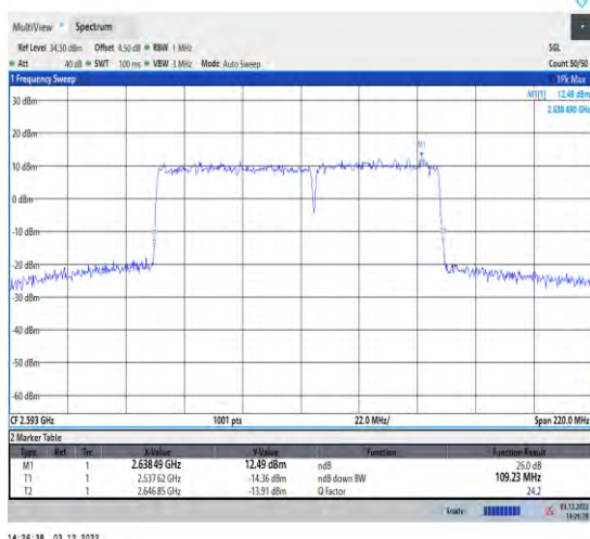
1-41-41-60+50-M-3-DFT-16QAM-Outer_Full
