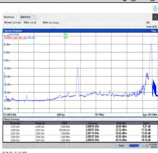
1-41-41-30-100+80-H-2-DFT-QPSK-Edge_1RB_Right
