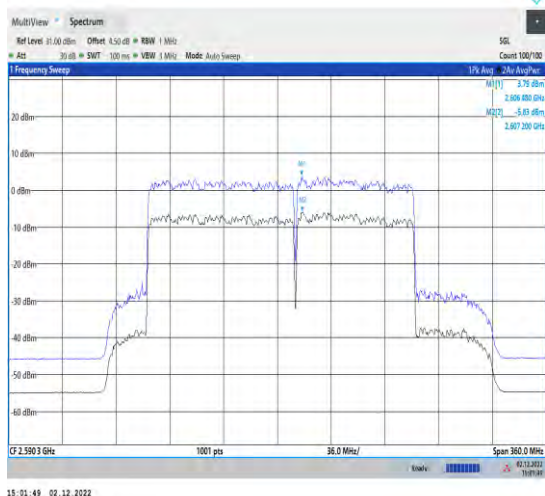
1-41-41-30-100+800+80-M-1-DFT-256QAM-Outer_Ful l-270@0-Ant1-9.73-100%-0.00-9.73-PASS-≤13
