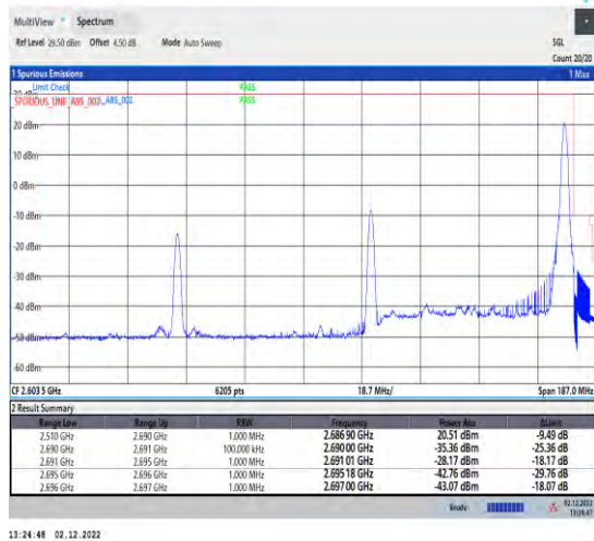
1-41-41-30-80+50-H-2-DFT-QPSK-Edge_1RB_Right
