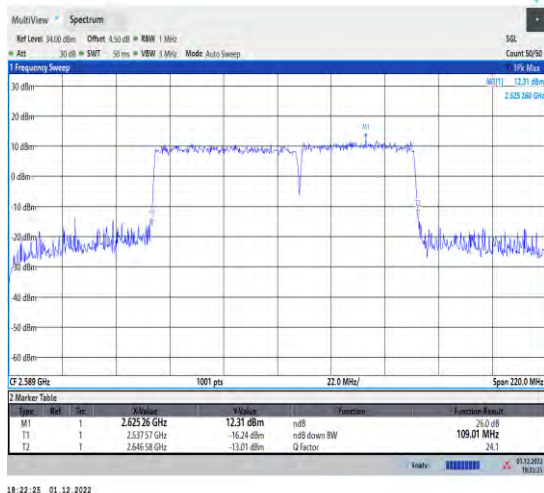
1-41-41-60+50-M-3-DFT-QPSK-Outer_Full
