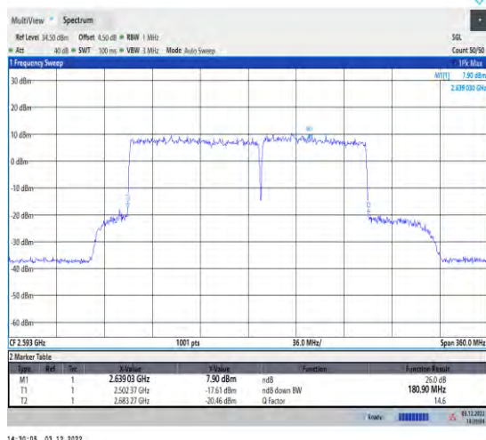
1-41-41-100+80-M-6-DFT-16QAM-Outer_Full
