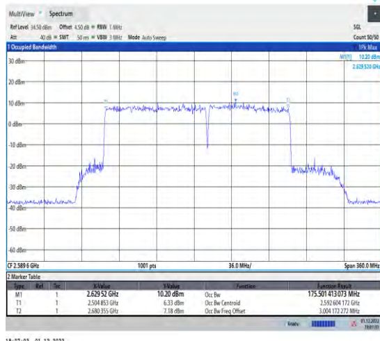
1-41-41-100+80-M-6-DFT-QPSK-Outet_Full
