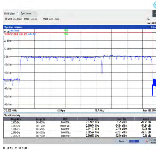
1-41-41-30-100+60-H-L-3-DFT-QPSK-Outer_Full
