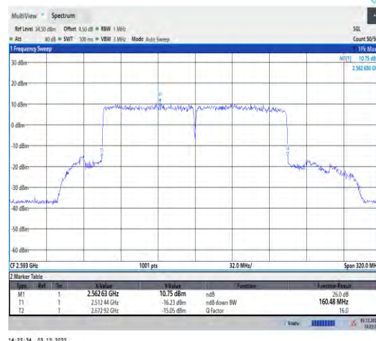
1-41-41-80+80-M-1-DFT-16QAM-Outet_Full
