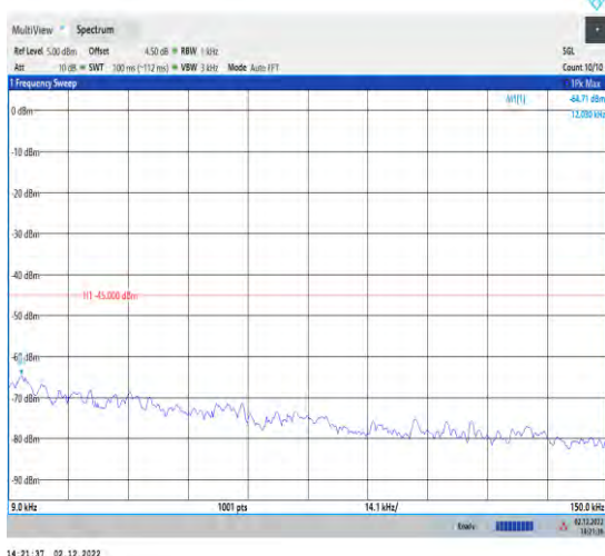
1-41-41-30-100-M-1-DFT-QPSK-Inner_1RB_Left-1 @1-0.009-0.15
