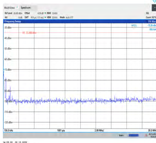
1-41-41-30-100-M-1-DFT-QPSK-Inner_1RB_Left-1@ 1-0.15-30
