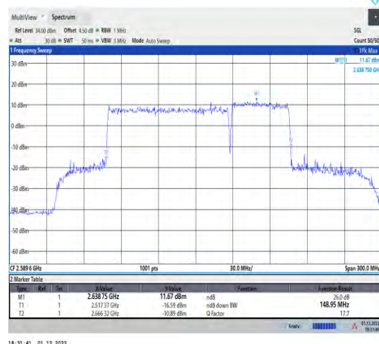
1-41-41-100+50-M-8-DFT-QPSK-Outer_Full
