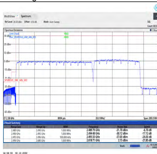
1-41-41-30-100+60-L-6-CP-QPSK-Outer_Full
