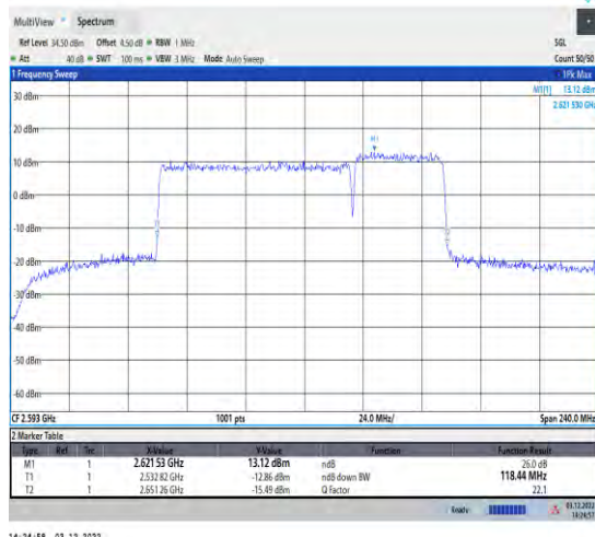
1-41-41-80+40-M-9-DFT-16QAM-Outet_Full
