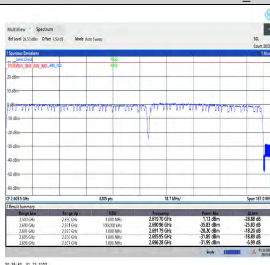
1-41-41-30-100+80-H-3-DFT-QPSK-Outer_Full
