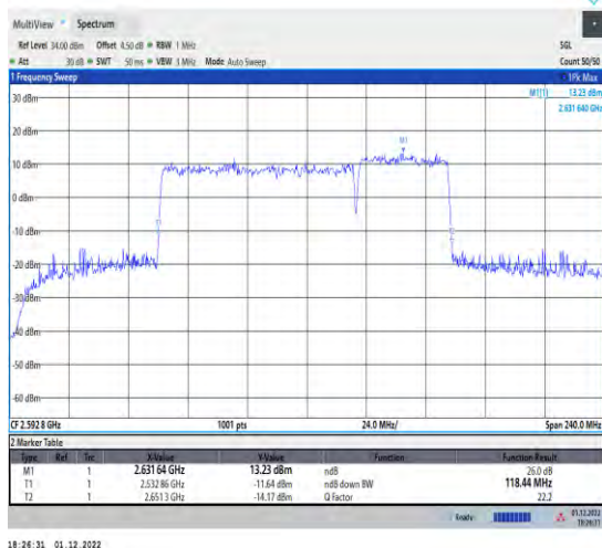
1-41-41-80+40-M-9-DFT-QPSK-Outer_Full
