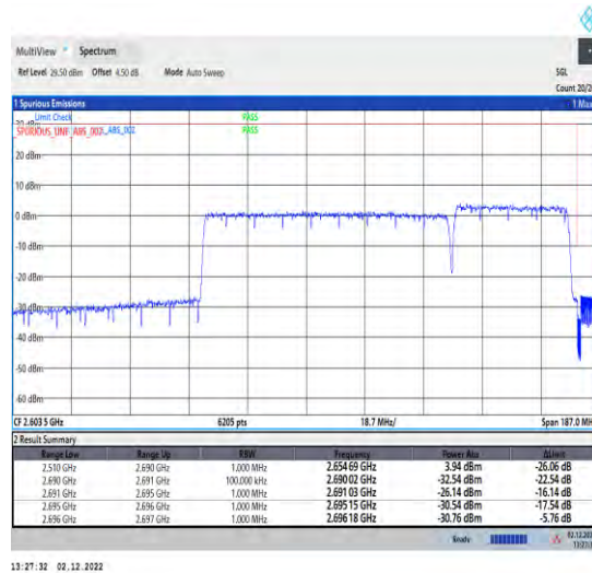
1-41-41-30-80+40-H-6-CP-QPSK-Outer_Full
