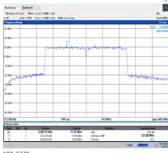
1-41-41-60+60-M-6-DFT-16QAM-Outer_Full
