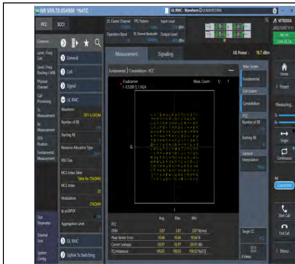
1-41-41-30-100-M-5-DFT-256QAM-Outer_Full-270@0-Ant1-see graph-PASS
