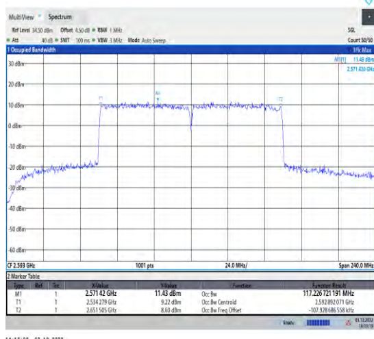
1-41-41-60+60-M-6-DFT-16QAM-Outet_Full
