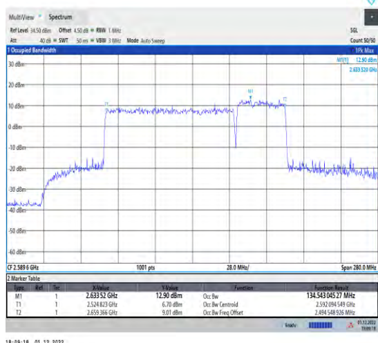
1-41-41-100+40-M-5-DFT-QPSK-Outer_Full
