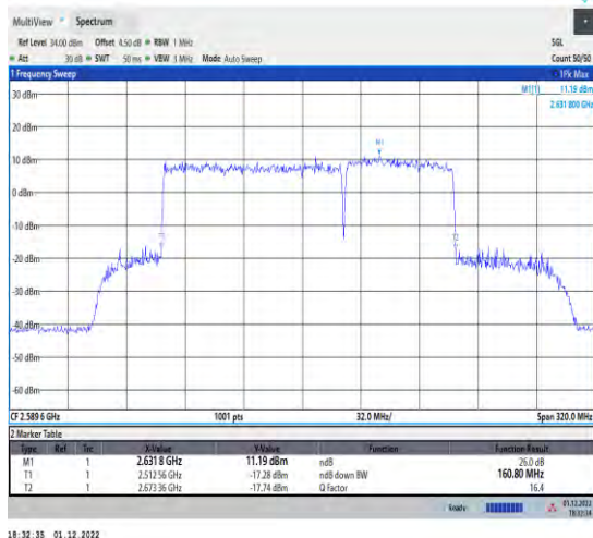
1-41-41-100+60-M-3-DFT-16QAM-Outer_Full
