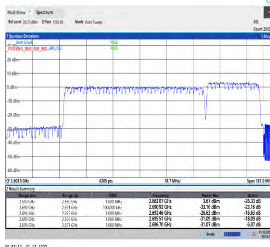
1-41-41-30-100+40-H-3-DFT-QPSK-Outer_Full
