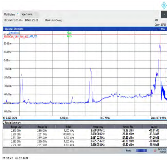
1-41-41-30-100+60-H-1-DFT-QPSK-Edge_1RB_Right
