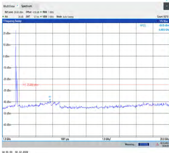
1-41-41-30-100-M-1-DFT-QPSK-Inner_1RB_Left-1 @1-1000-20000
