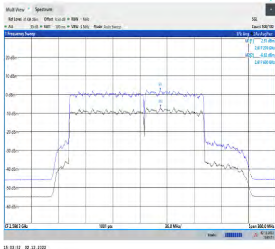
1-41-41-30-100+80-L-1-DFT-256QAM-Outer_Full-270 @0-Ant1-9.53-100%-0.00-9.53-PASS-≤13
