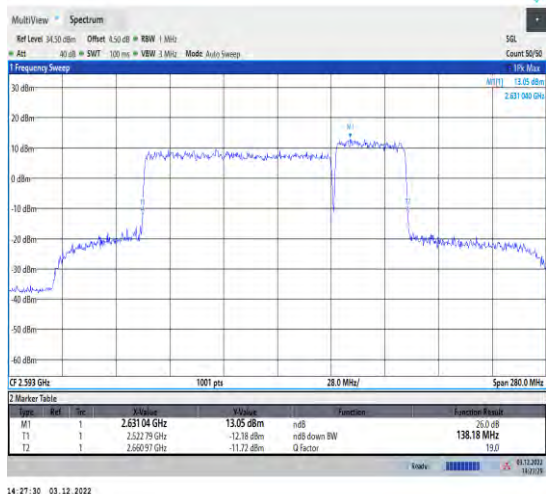
1-41-41-100+40-M-5-DFT-16QAM-Outer_Full
