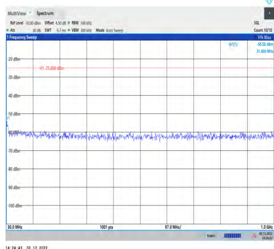
1-41-41-30-100-M-1-DFT-QPSK-Inner_1RB_Left-1@ 1-30-1000
