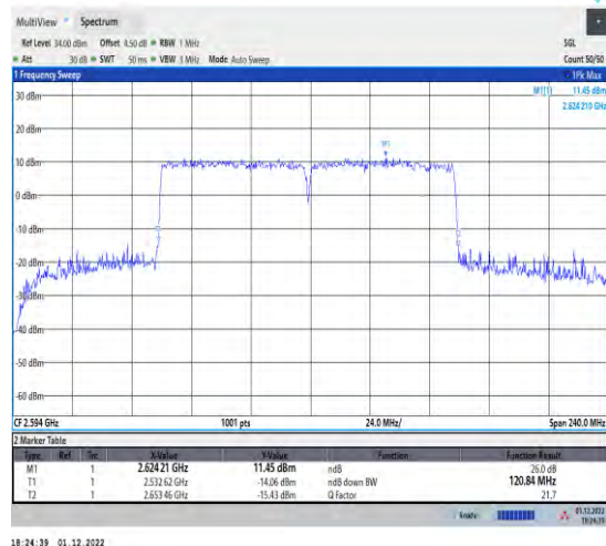
1-41-41-60+60-M-6-DFT-QPSK-Outer_Full
