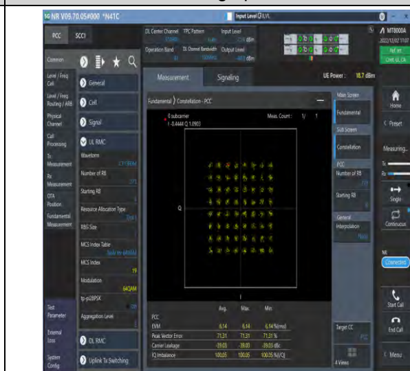
1-41-41-30-100-M-8-CP-64QAM-Outer_Full-273@0-Ant1-see graph-PASS
