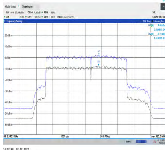
1-41-41-30-100+80-M-2-CP-256QAM-Outer_Full-2 73@0-Ant1-9.29-100%-0.00-9.29-PASS-≤13
