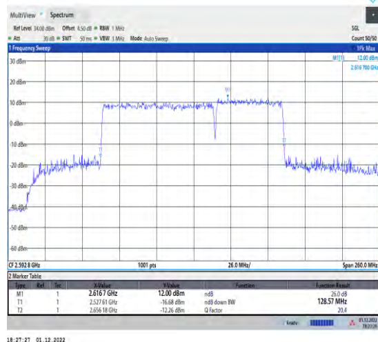
1-41-41-80+50-M-4-DFT-QPSK-Outer_Full
