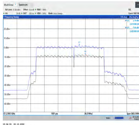
1-41-41-30-100-L-2-CP-256QAM-Outer_Full-273@ 0-Ant1-9.53-100%-0.00-9.53-PASS-≤13
