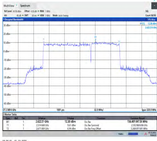
1-41-41-100+60-M-3-DFT-QPSK-Outet_Full
