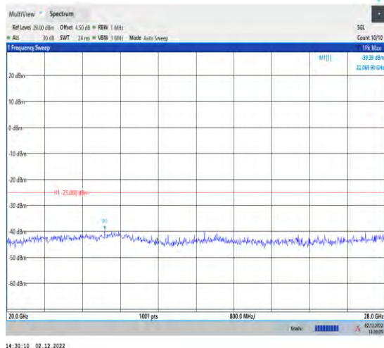
1-41-41-30-100-L-1-DFT-QPSK-Inner_1RB_Left-1@ 1-20000-28000
