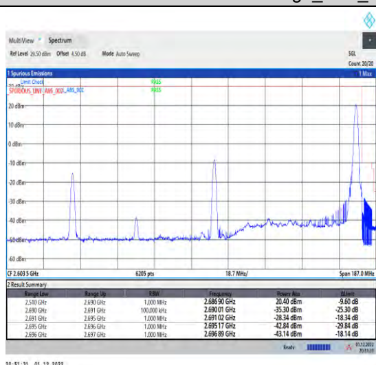
1-41-41-30-100+50-H-2-DFT-QPSK-Edge_1RB_Right
