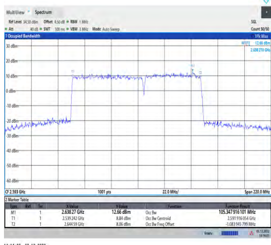
1-41-41-60+50-M-3-DFT-16QAM-Outet_Full
