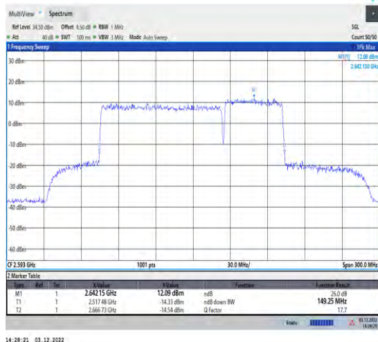
1-41-41-100+50-M-8-DFT-16QAM-Outer_Full
