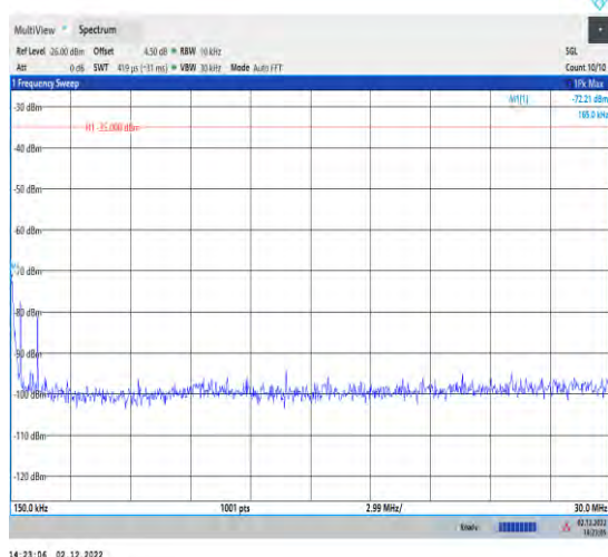
1-41-41-30-100-M-1-DFT-QPSK-Inner_1RB_Left-1 @1-0.15-30
