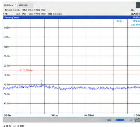
1-41-41-30-100-M-1-DFT-QPSK-Inner_1RB_Left-1@ 1-20000-28000
