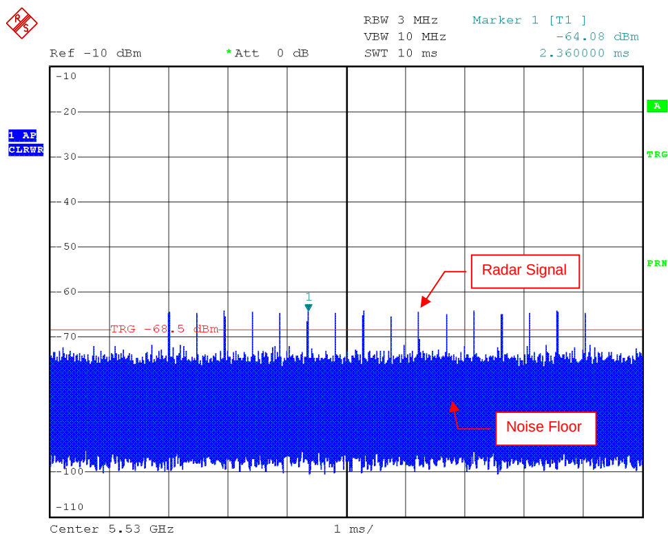
Radar Signal 3
