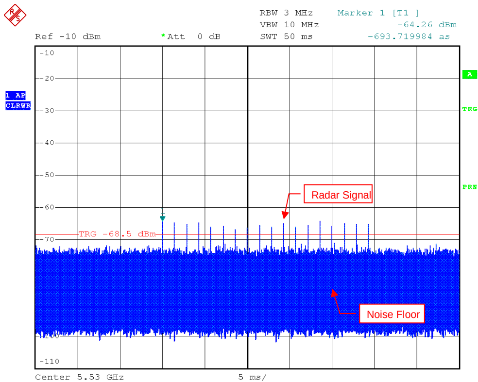
Radar Signal 0
