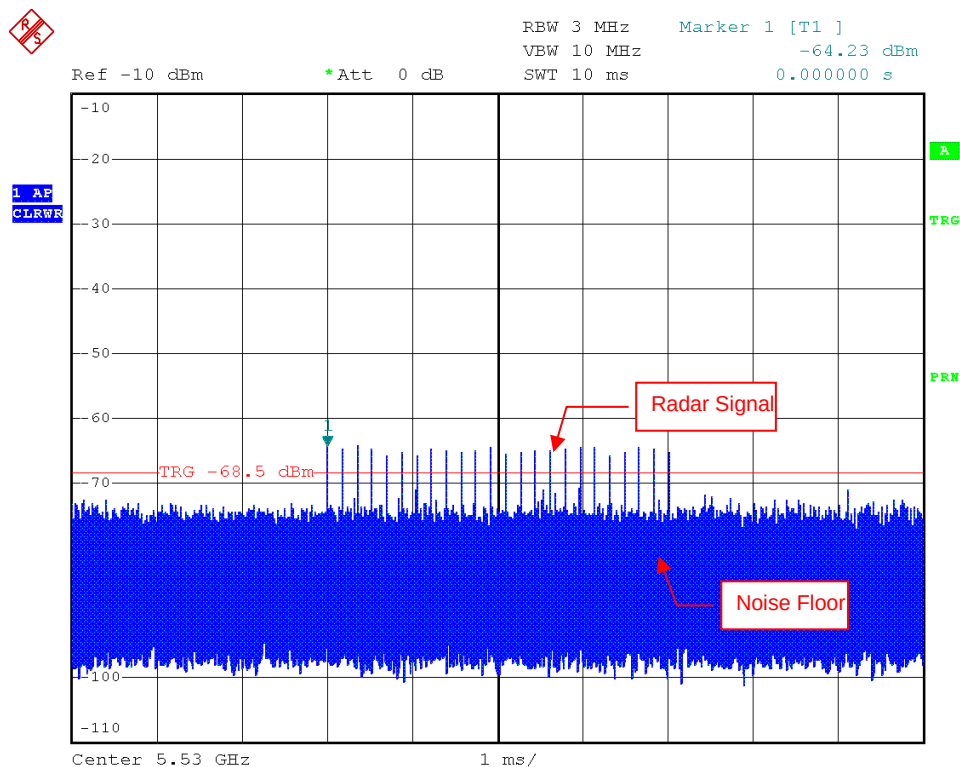
Radar Signal 2
