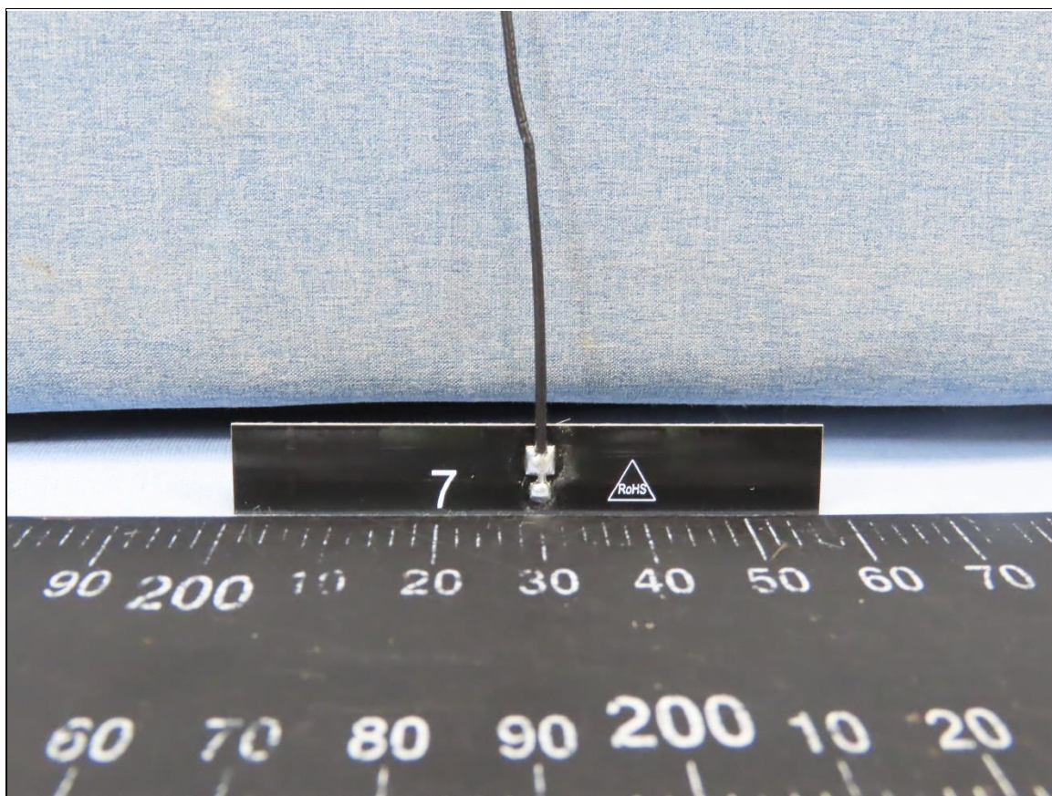
ANT7 Antenna
