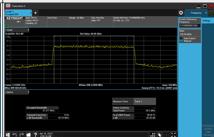
BPSK CH 634666 (3519.99 MHz)
